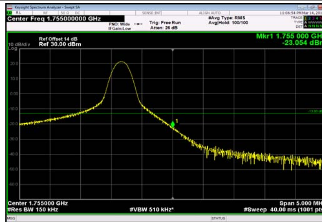
HighRange_FDD04_15MHz_1747.5_fullRB _High_QPSK
