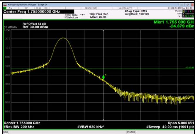
HighRange_FDD04_20MHz_1745_OneRB _high_Q16
