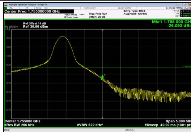
HighRange_FDD04_20MHz_1745_OneRB _high_QPSK
