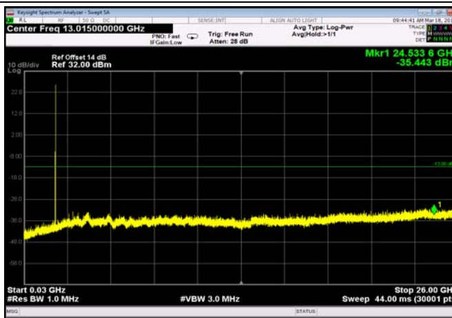
FDD02_HighRange_15MHz_30MHz~26GHz
