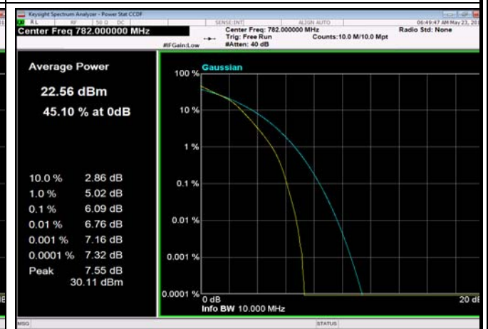
FDD13_10MHz_782MHz_fullRB_Q16
