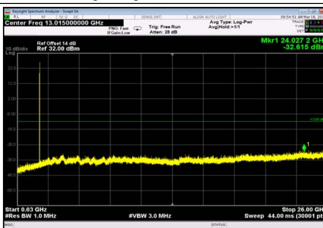
FDD02_HighRange_3MHz_30MHz~26GHz
