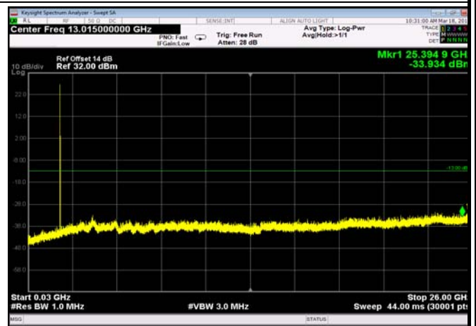
FDD02_HighRange_20MHz_30MHz~26GHz
