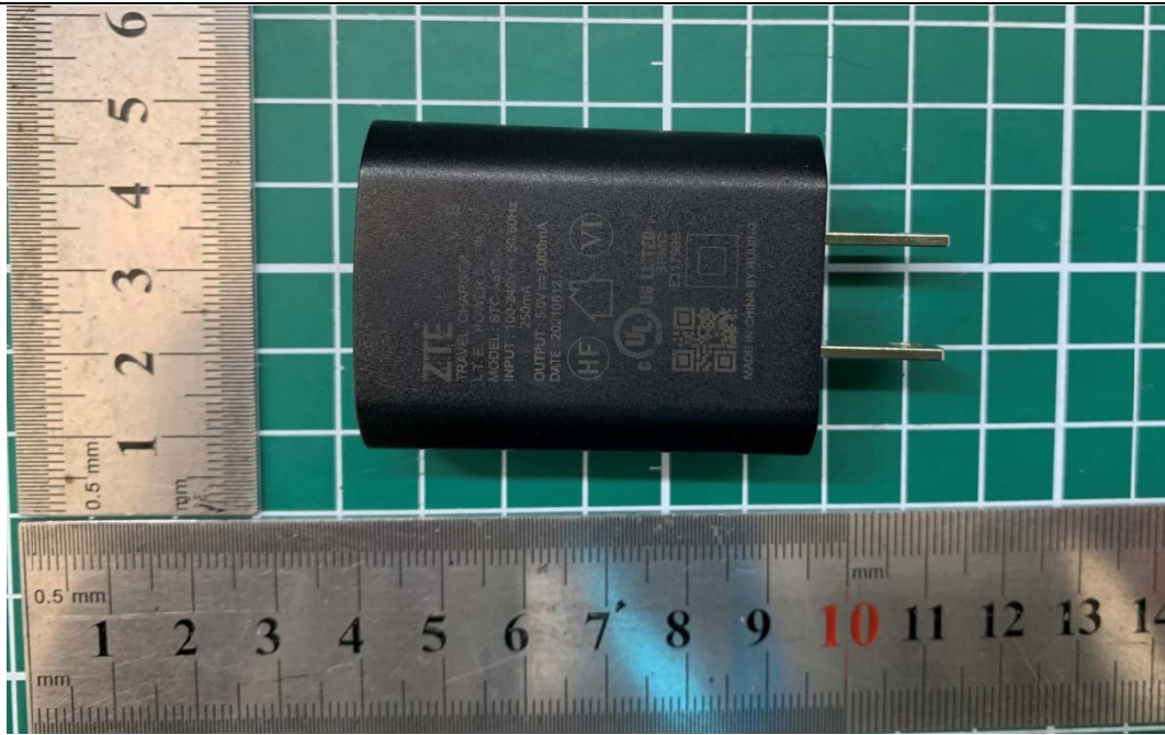
b: Adapter
