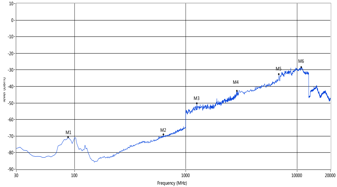
RSE Test case_FCC_FCC PART 24
