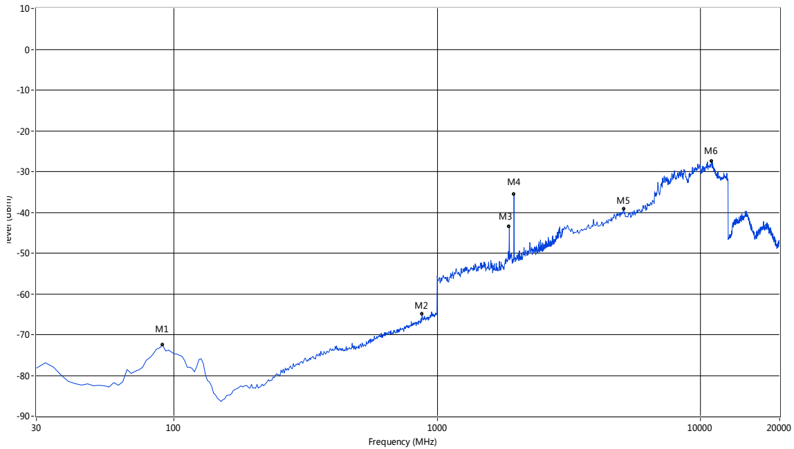
RSE Test case_FCC_FCC PART 24
