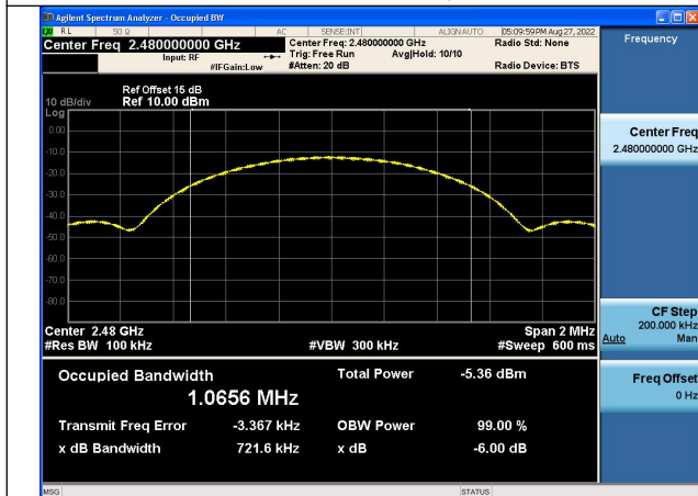
Test Mode:GFSK (LE 1Mbps) 2480MHz
