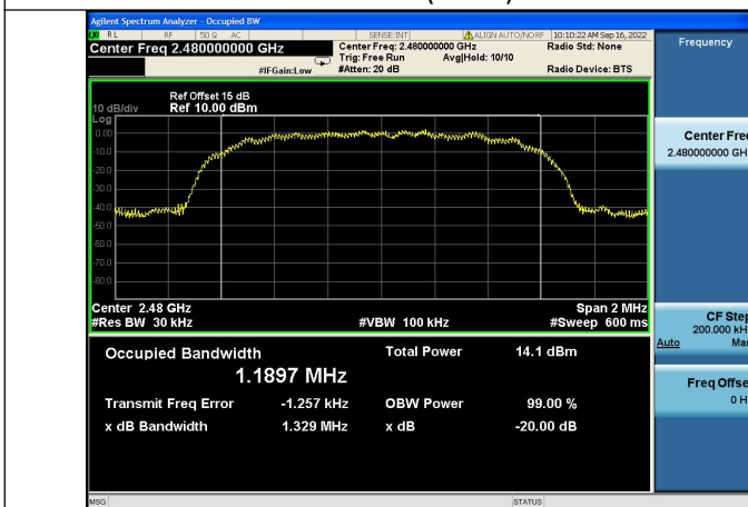
Test Mode:8DPSK(3DH5) 2480MHz
