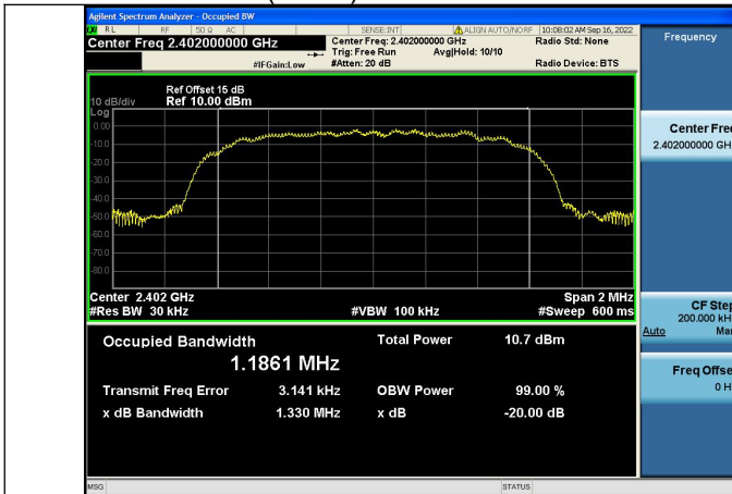
Test Mode:8DPSK(3DH5) 2402MHz
