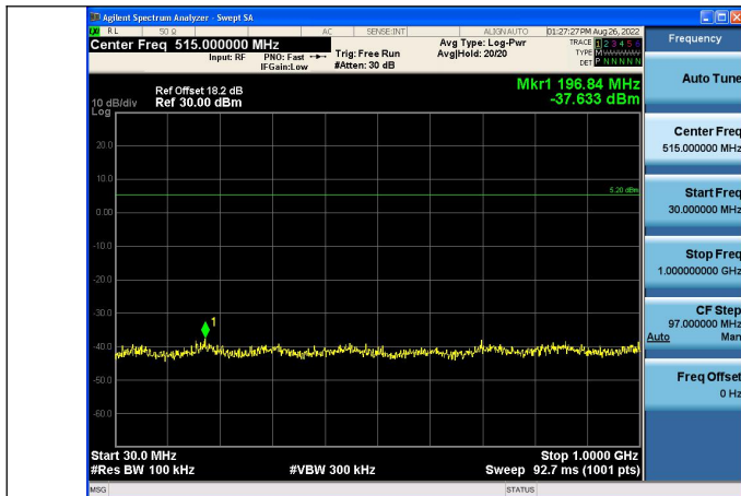
Channel 9262 30MHz~1GHz(dBm)
