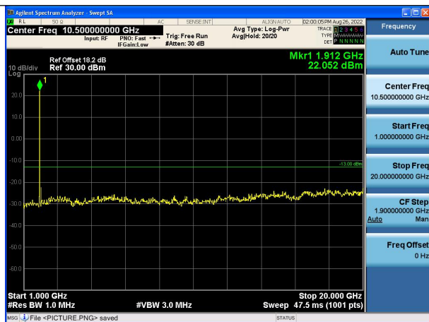
Channel 9262 1GHz~20GHz(dBm)
