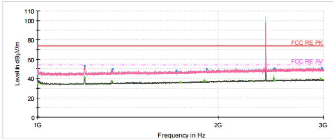
Note: The signal beyond the limit is carrier. Radiates Emission from 1GHz to 3GHz
