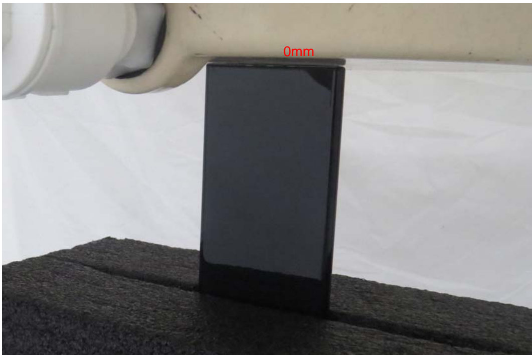
Picture 18: Bottom Edge, the distance from handset to the bottom of the Phantom is 0mm
