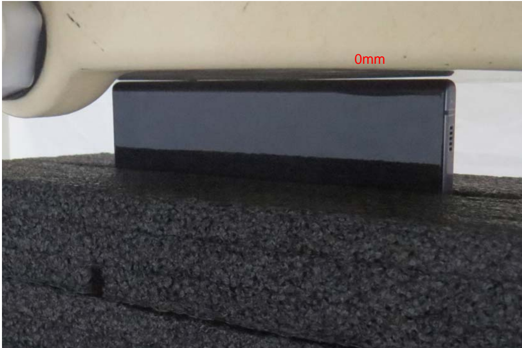
Picture 15: Left Edge, the distance from handset to the bottom of the Phantom is 0mm
