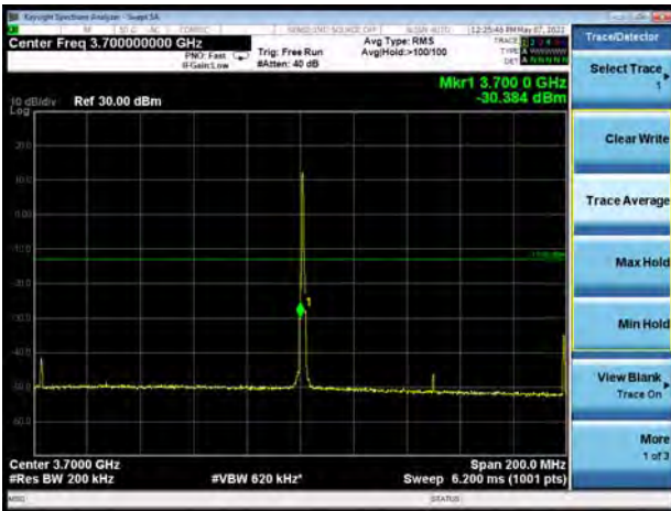
NR n77 subset 2 P1/2 BPSK 100MHz CH-Low 100%RB
