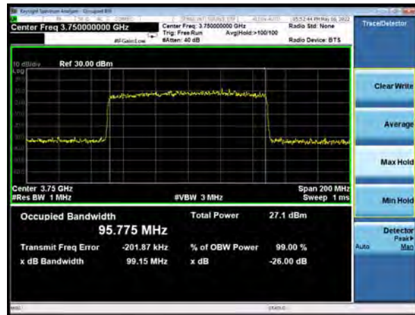
DC_2A-n77(subset 2)AQPSK 100%RB 100MHz CH-Middle
