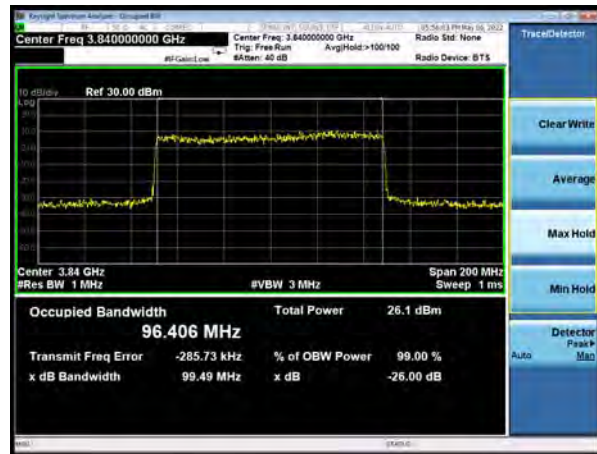
DC_2A-n77(subset 2)A QPSK 100%RB 100MHz CH-High
