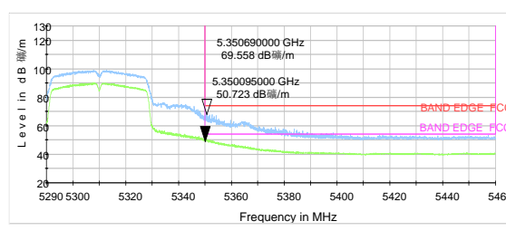
802.11ac VHT20 -Channel 64: Peak + Average
