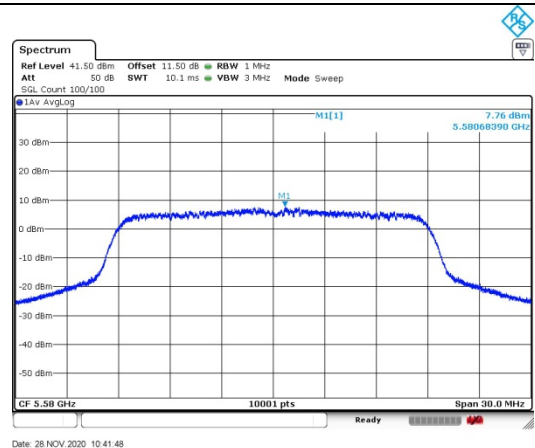
Test Mode: 802.11n HT20 Chain0
