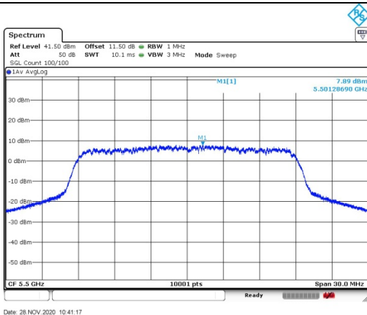
Test Mode: 802.11n HT20 Chain0
