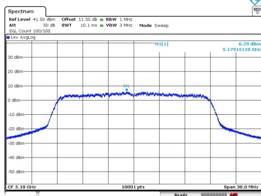
Test Mode: 802.11n HT20 Chain0
