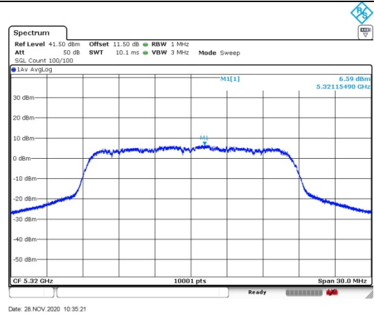
Test Mode: 802.11a Chain0
