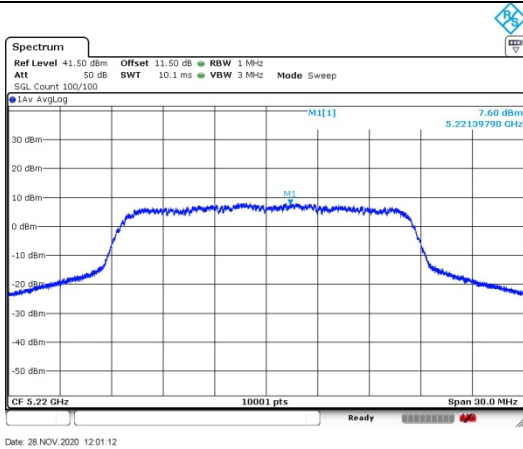
Test Mode: 802.11a Chain1
