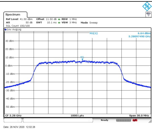
Test Mode: 802.11a Chain1
