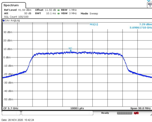
Test Mode: 802.11n HT20 Chain1
