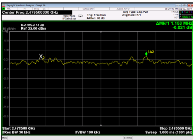
8DPSK,Hopping3DH5,2478.5~2480.5
