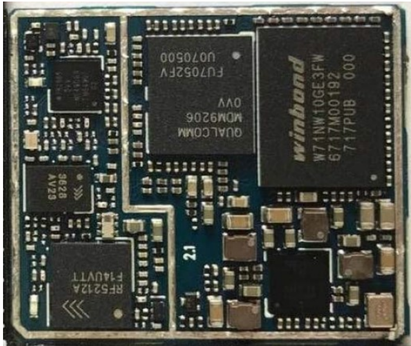
LTE Modular internal photo
