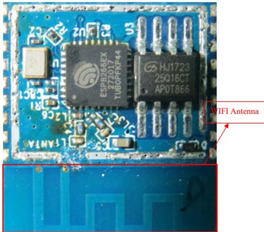
WiFi Modular Internal Photo
