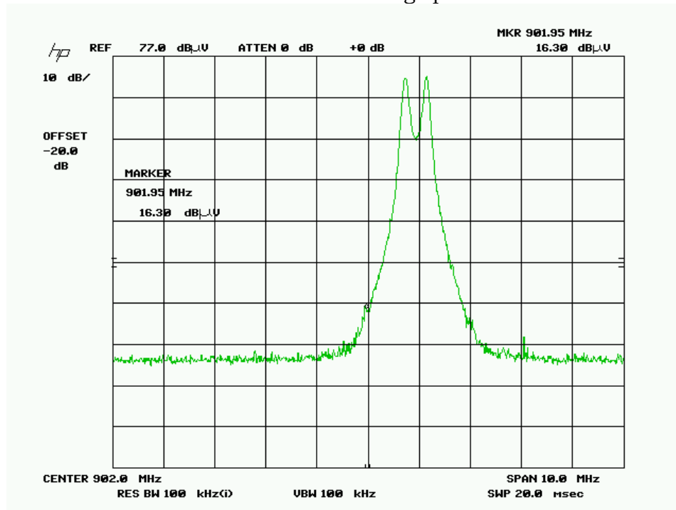
ch 902.94 -Lower band-edge peak - Horiz
