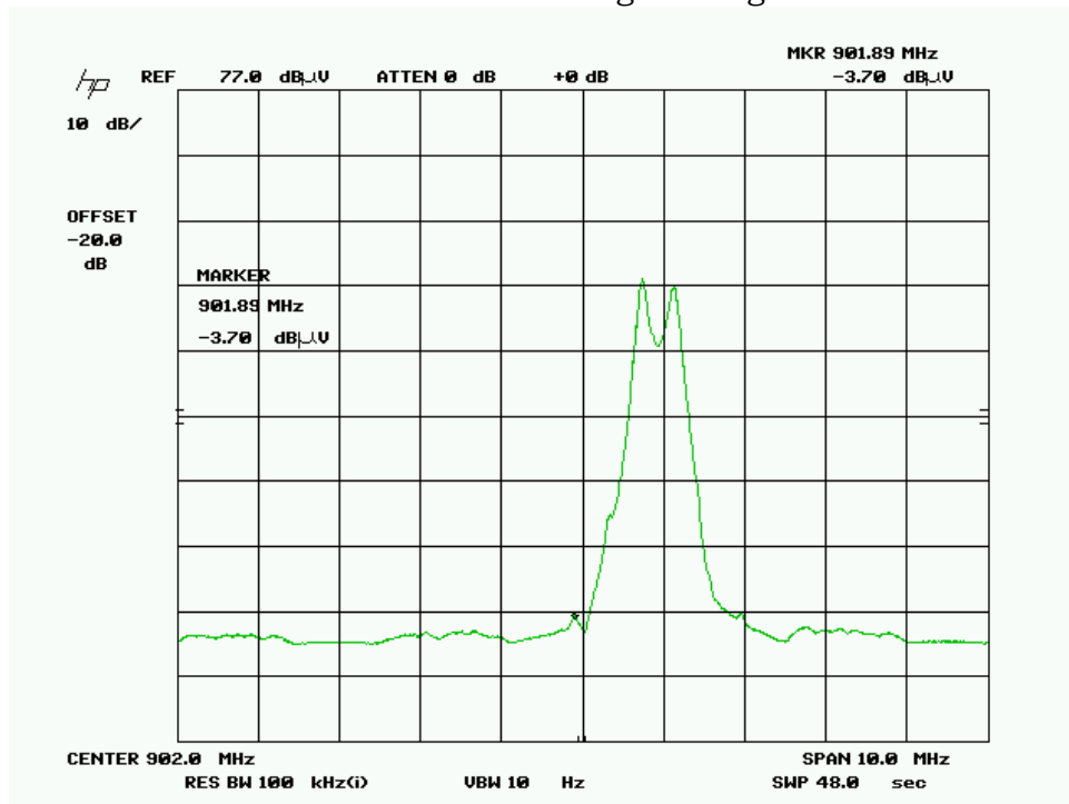
ch 902.94 -Lower band-edge average - Horiz
