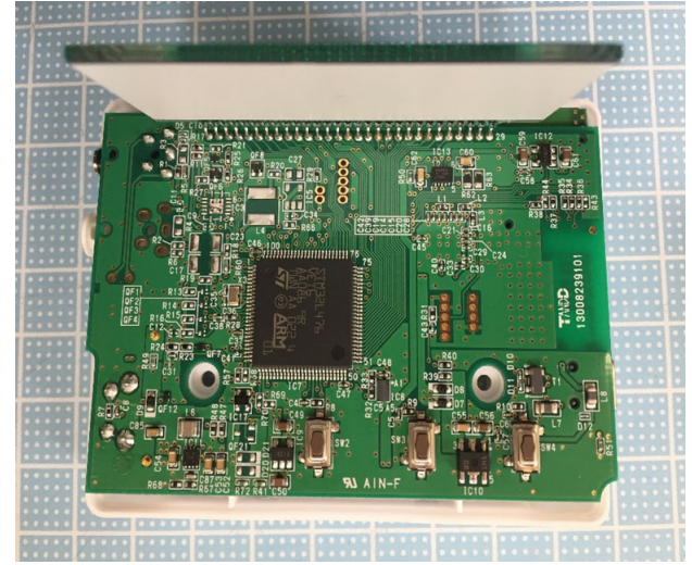
Board A side Inside of LCD
