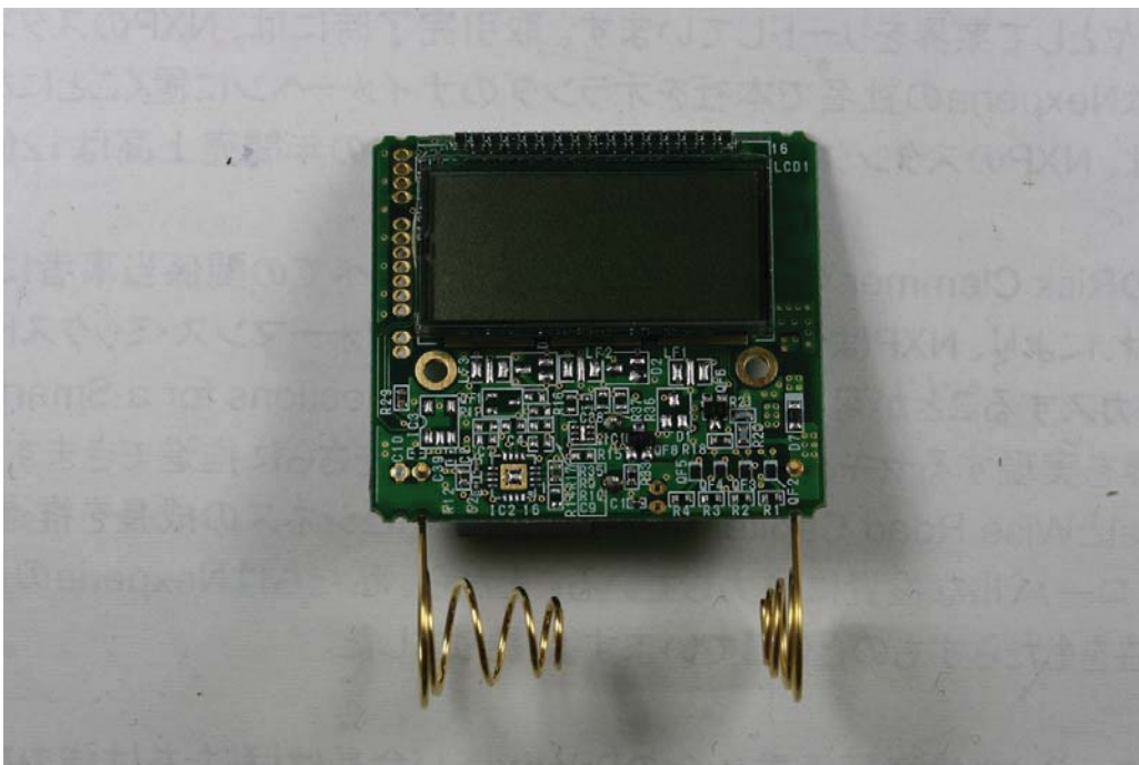
Cover Removed
