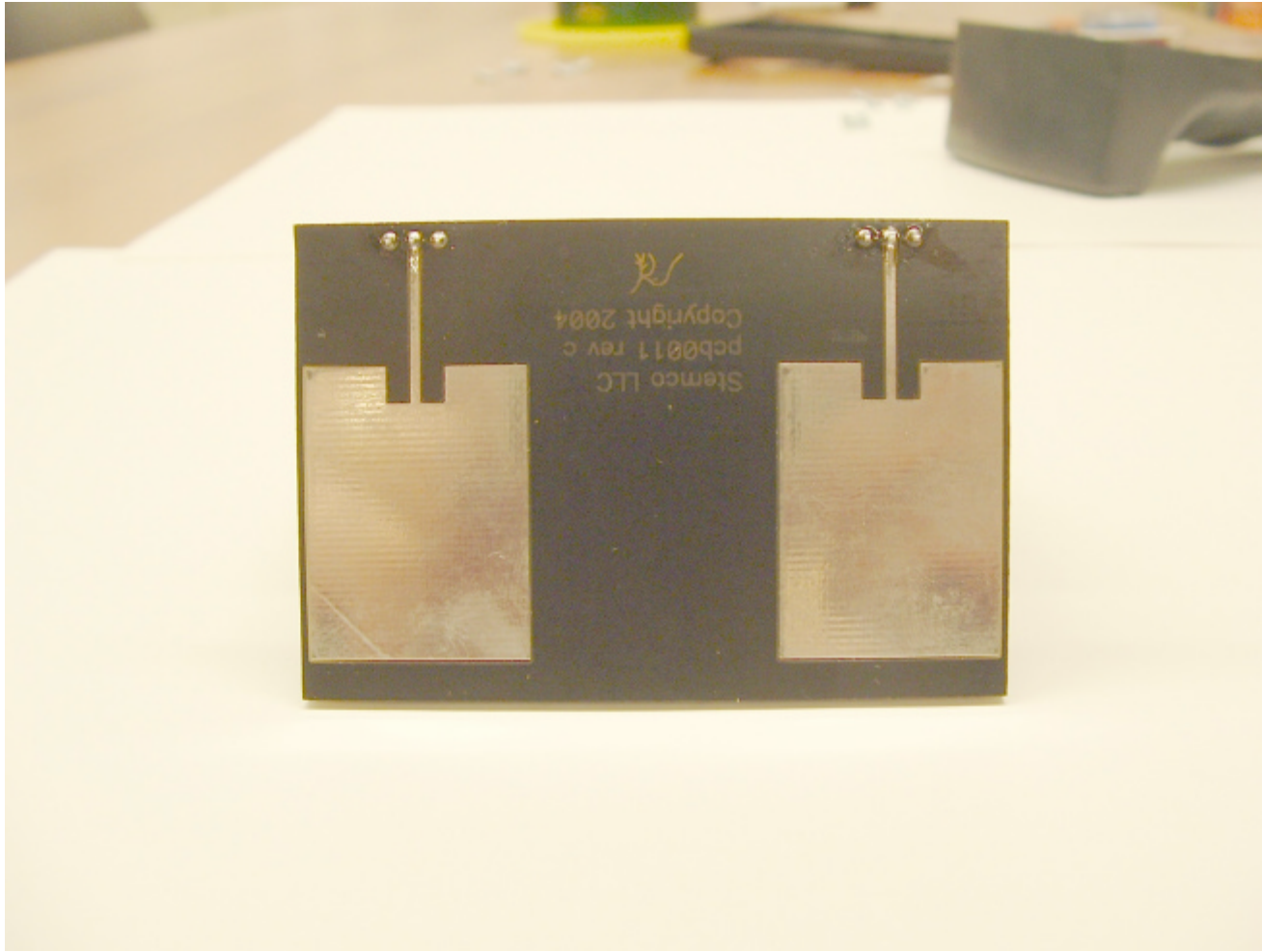
Antenna Board
