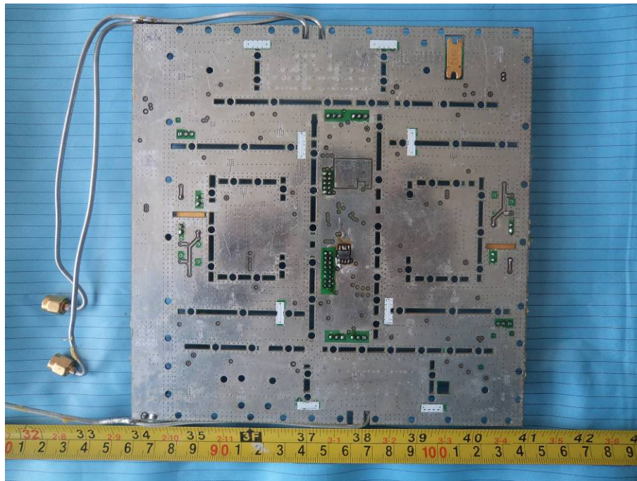
EUT – Main Unit Bottom Cover off View
