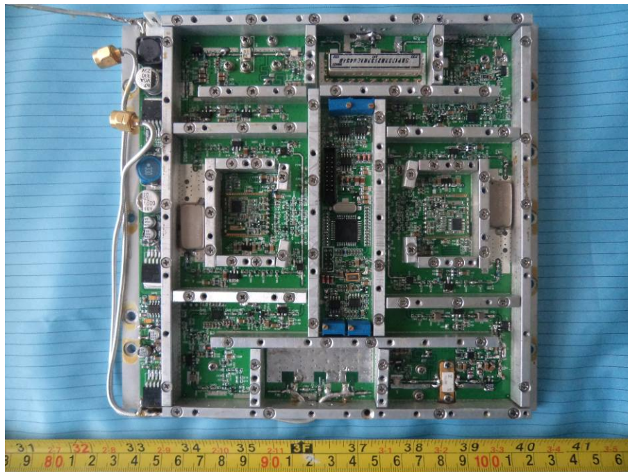
EUT – Main Unit Top Cover off View
