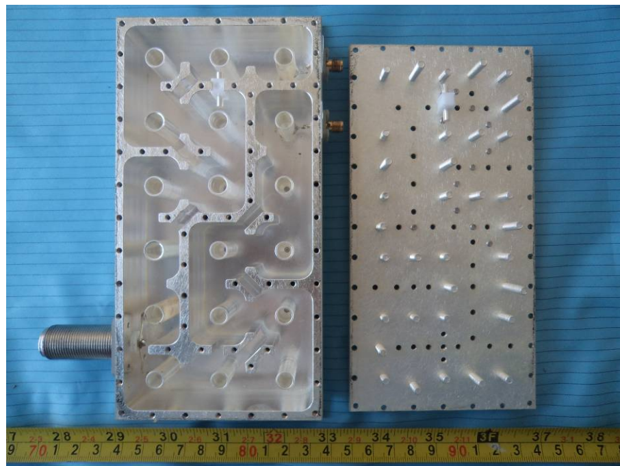
EUT –DUPLEXER Cover off View
