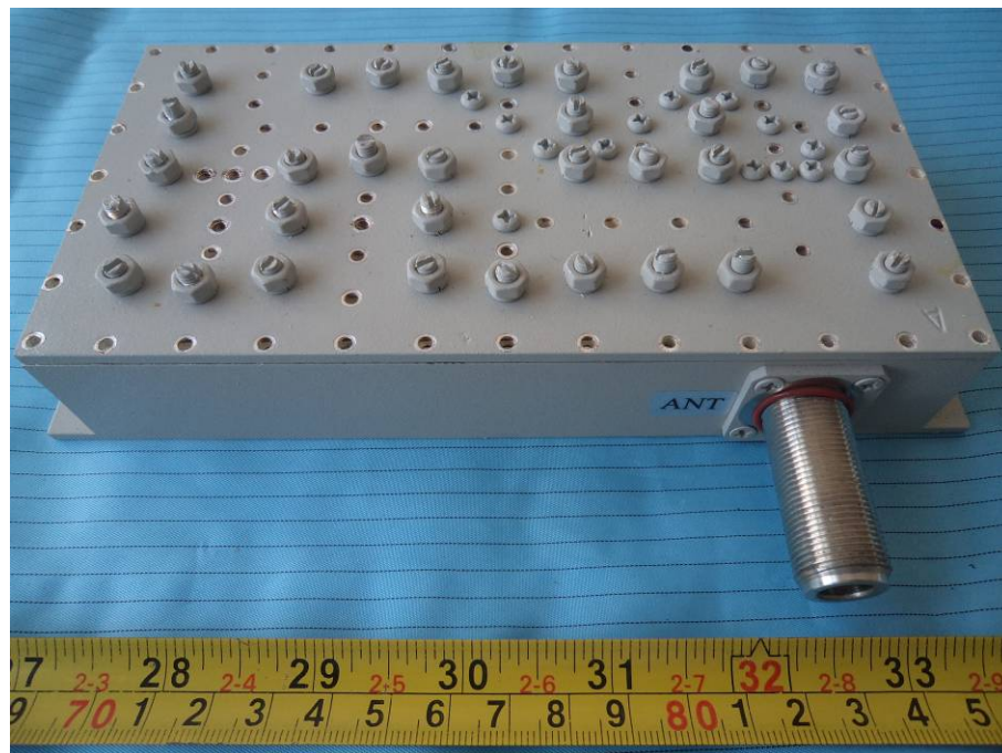
EUT –DUPLEXER Right Side View
