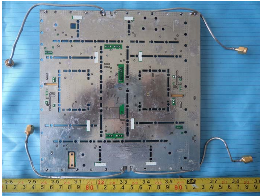
EUT –Main Unit 1 Bottom Cover off View
