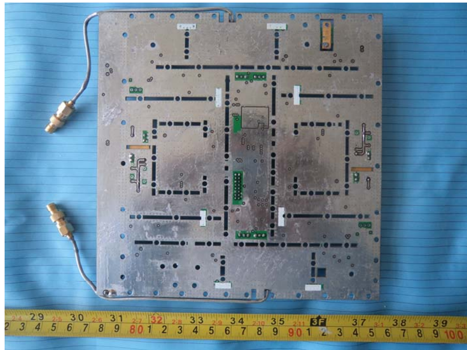
EUT –Main Unit 2 Bottom Cover off View
