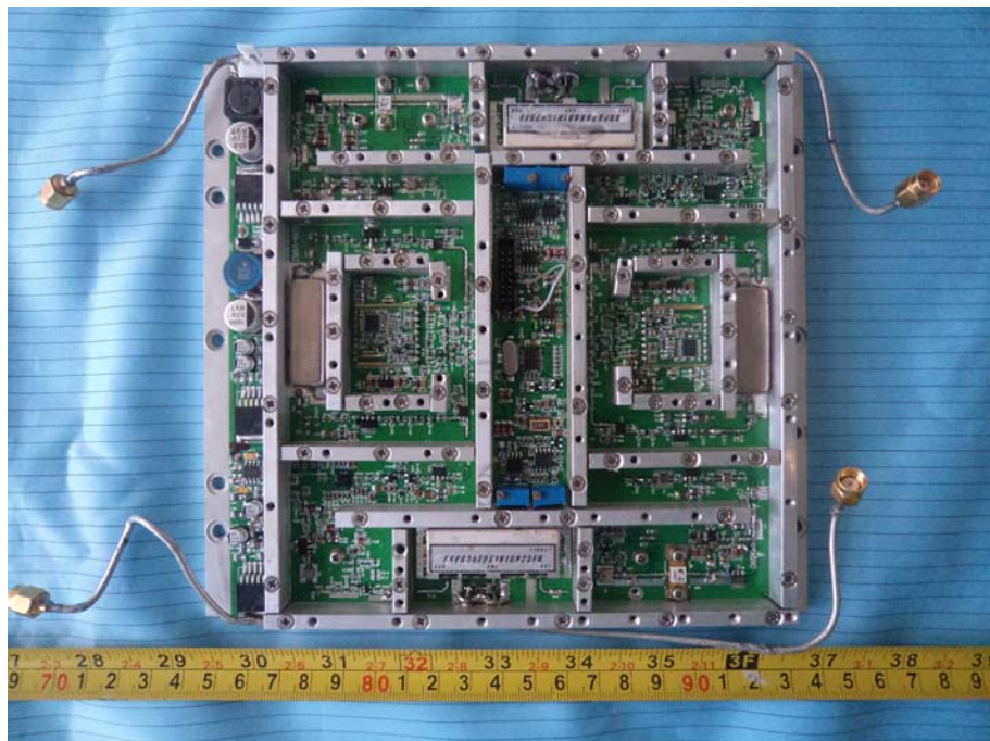
EUT –Main Unit 1 Top Cover off View
