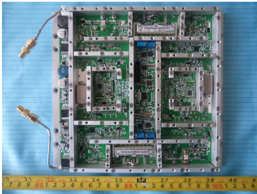
EUT –Main Unit 2 Top Cover off View
