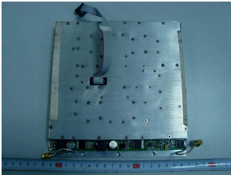
EUT – Main Board with Shieldong Cover Top View
