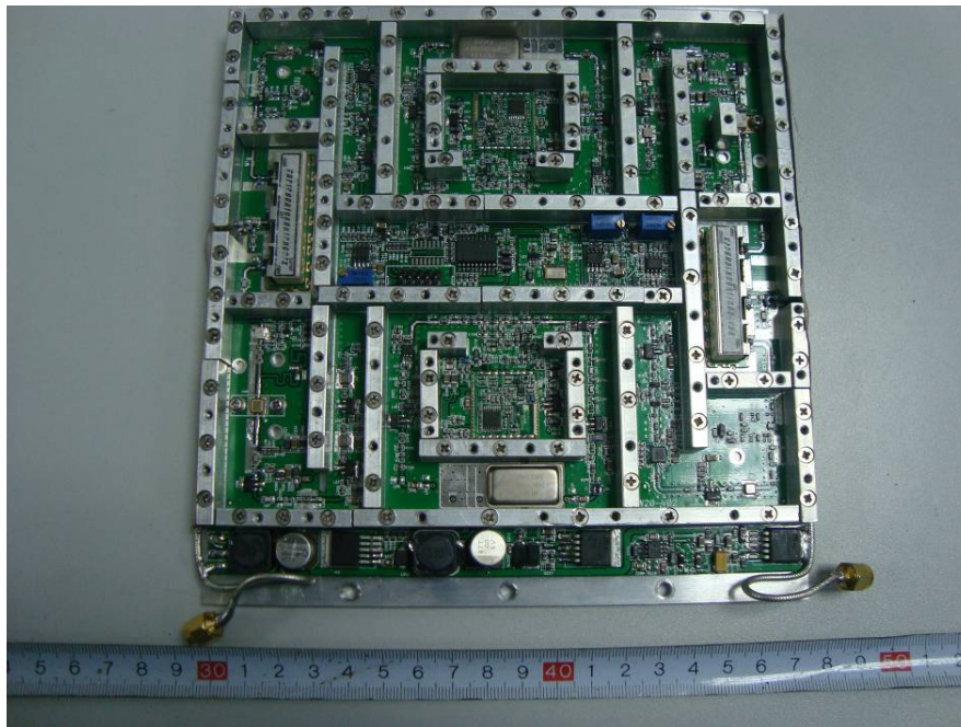
EUT – Main Main Top Shielding off View
