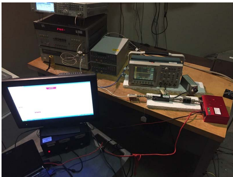
Transmit Transient Frequency Behaviour
