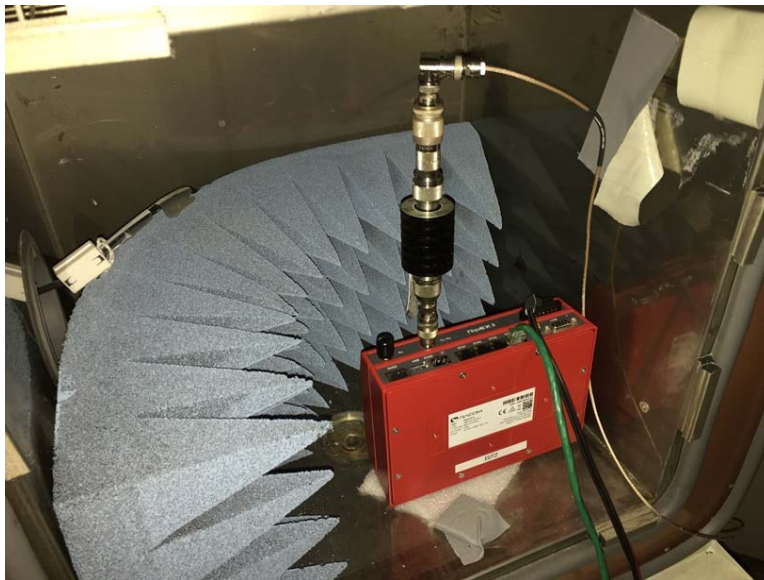
Frequency Stability, EUT
