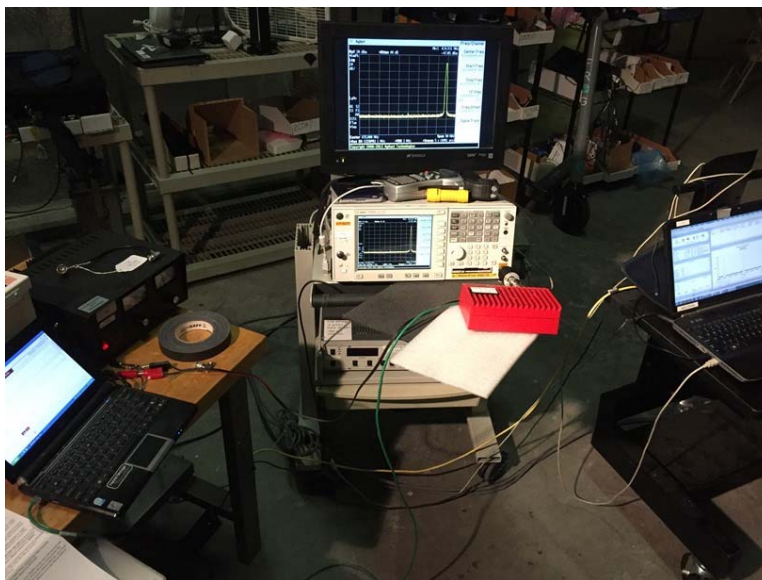
Conducted Antenna Port Measurements Power, Bandwidth, Mask, Spurious
