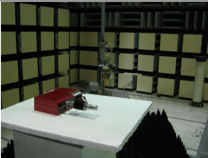
Radiated Emissions above 1 GHz, Front
