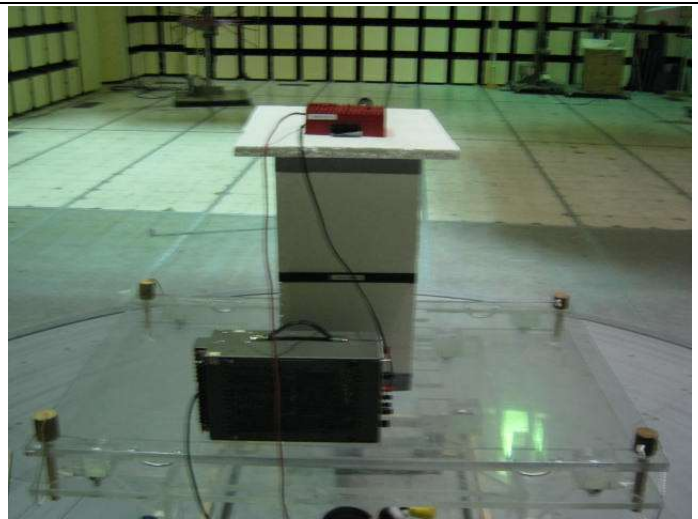
Radiated Emissions above 1 GHz, Back
