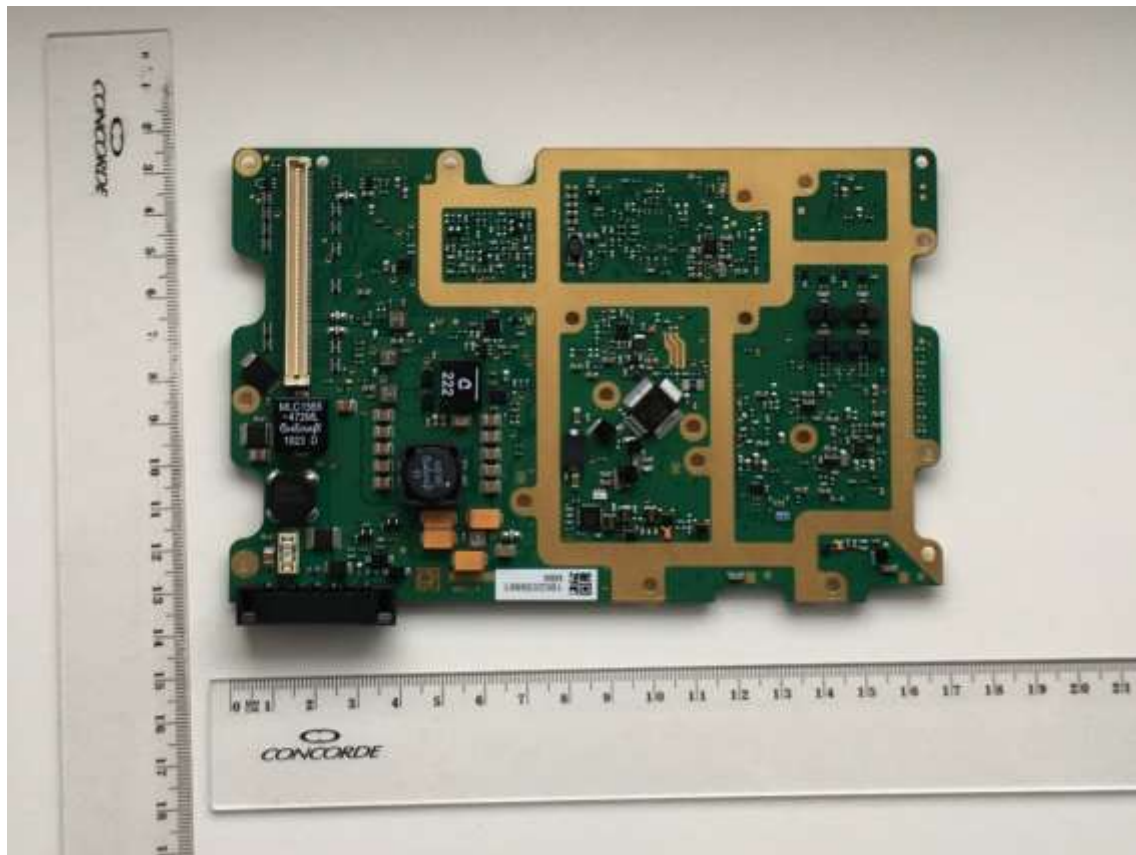
RF Board, Bottom
