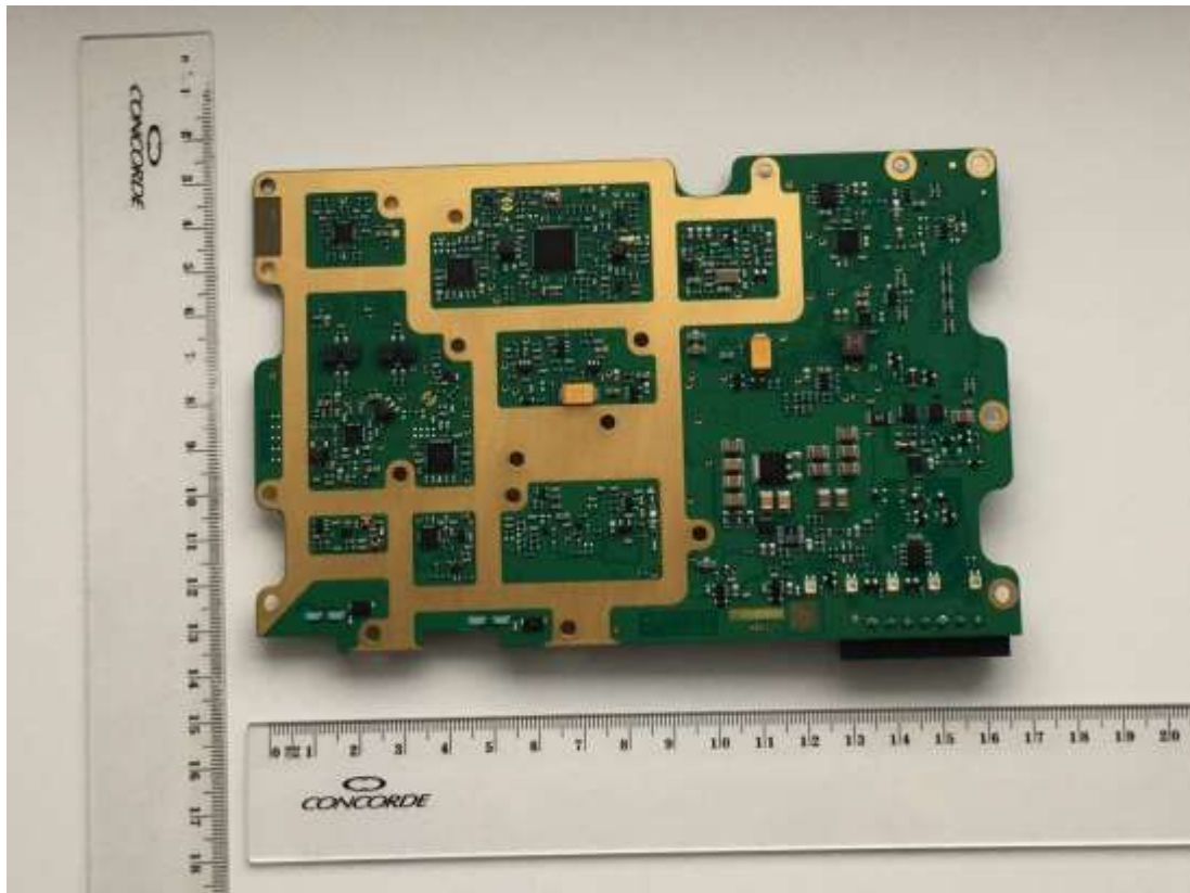
RF Board, Top
