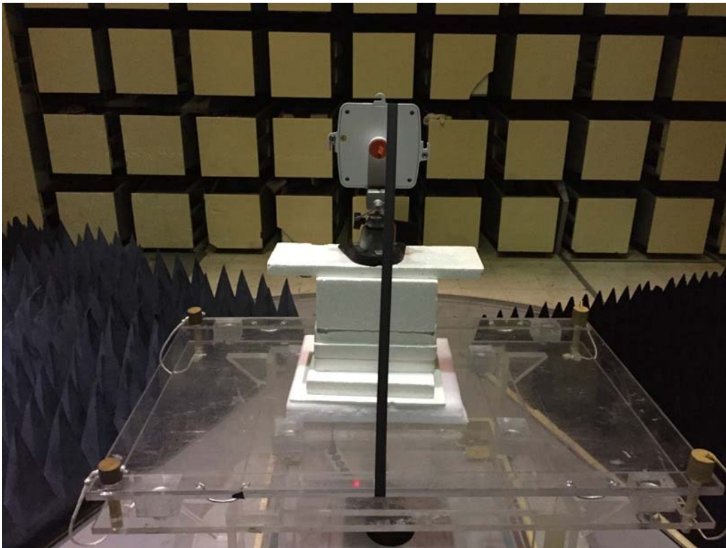
Radiated Emissions: 30 MHz to 18 GHz, Front
