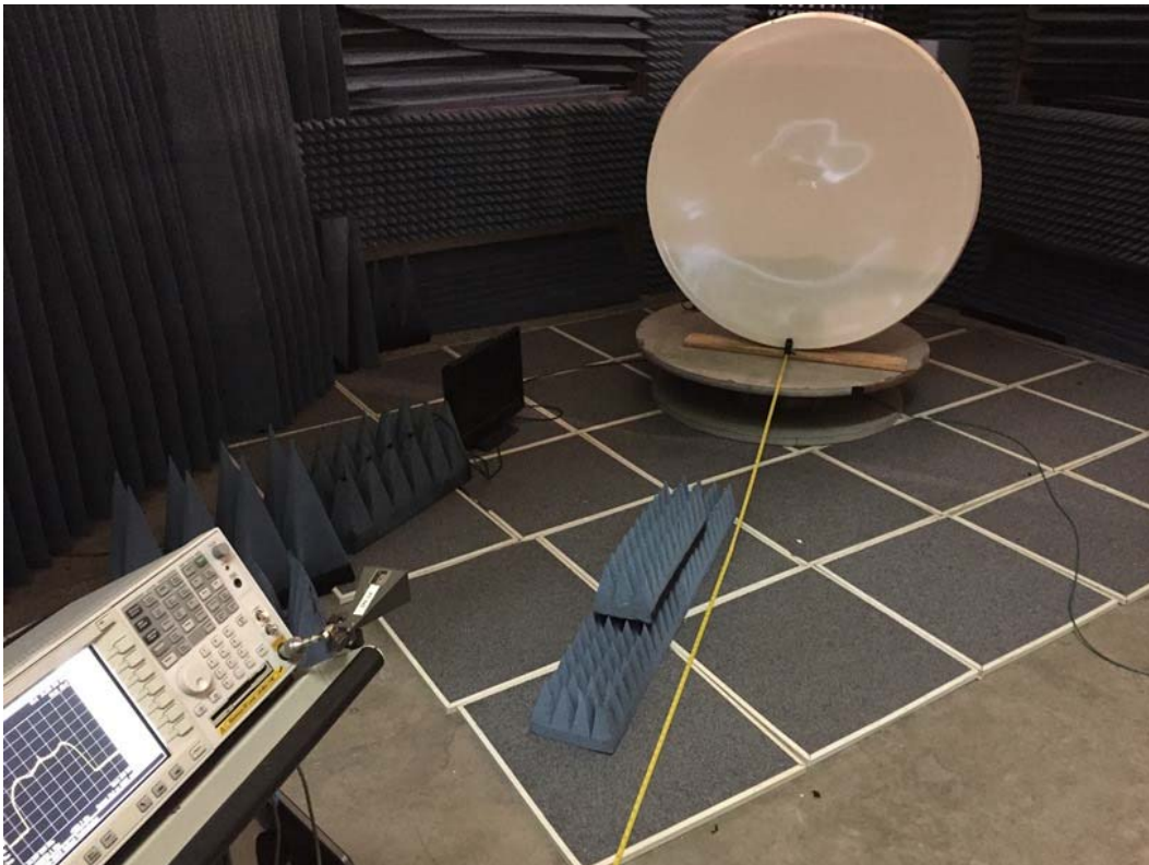
Radiated Emissions: Part 101.111
