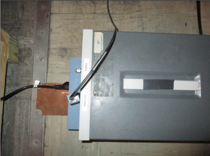
Conducted Emissions Neutral Line Test
