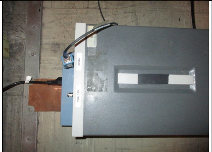
Conducted Emissions Phase Line Test
