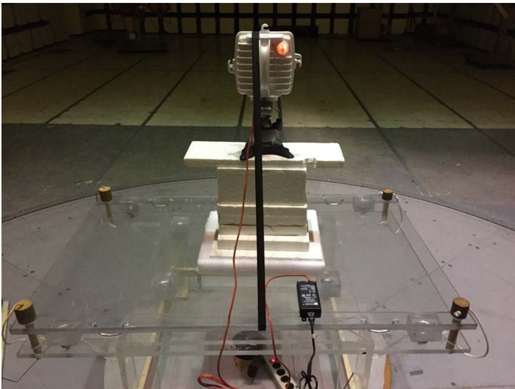
Radiated Emissions: 30 MHz to 18 GHz, Back
