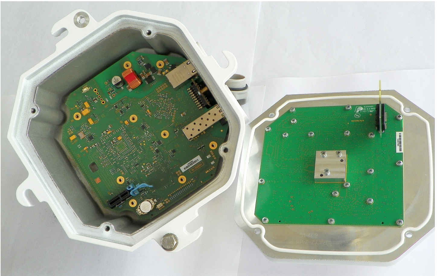
Initial Disassembly: Logic Board Left, RF Board Right, and small Extender Card
