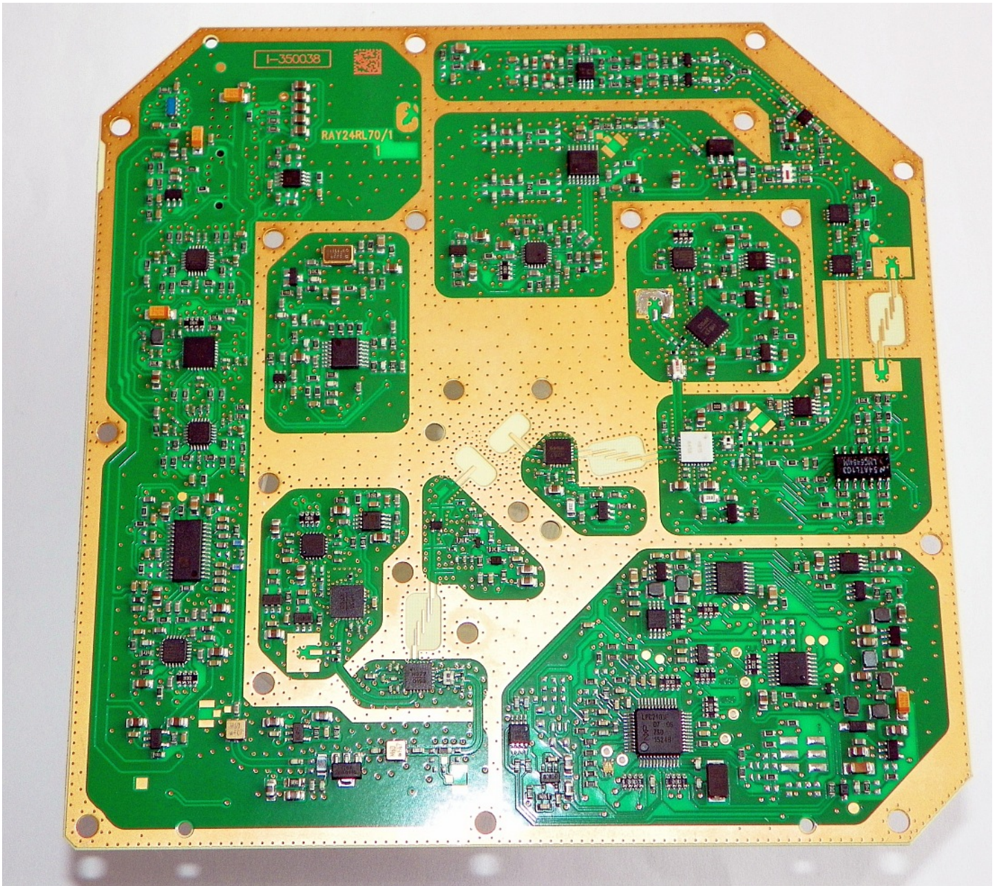
RF Board, Top
