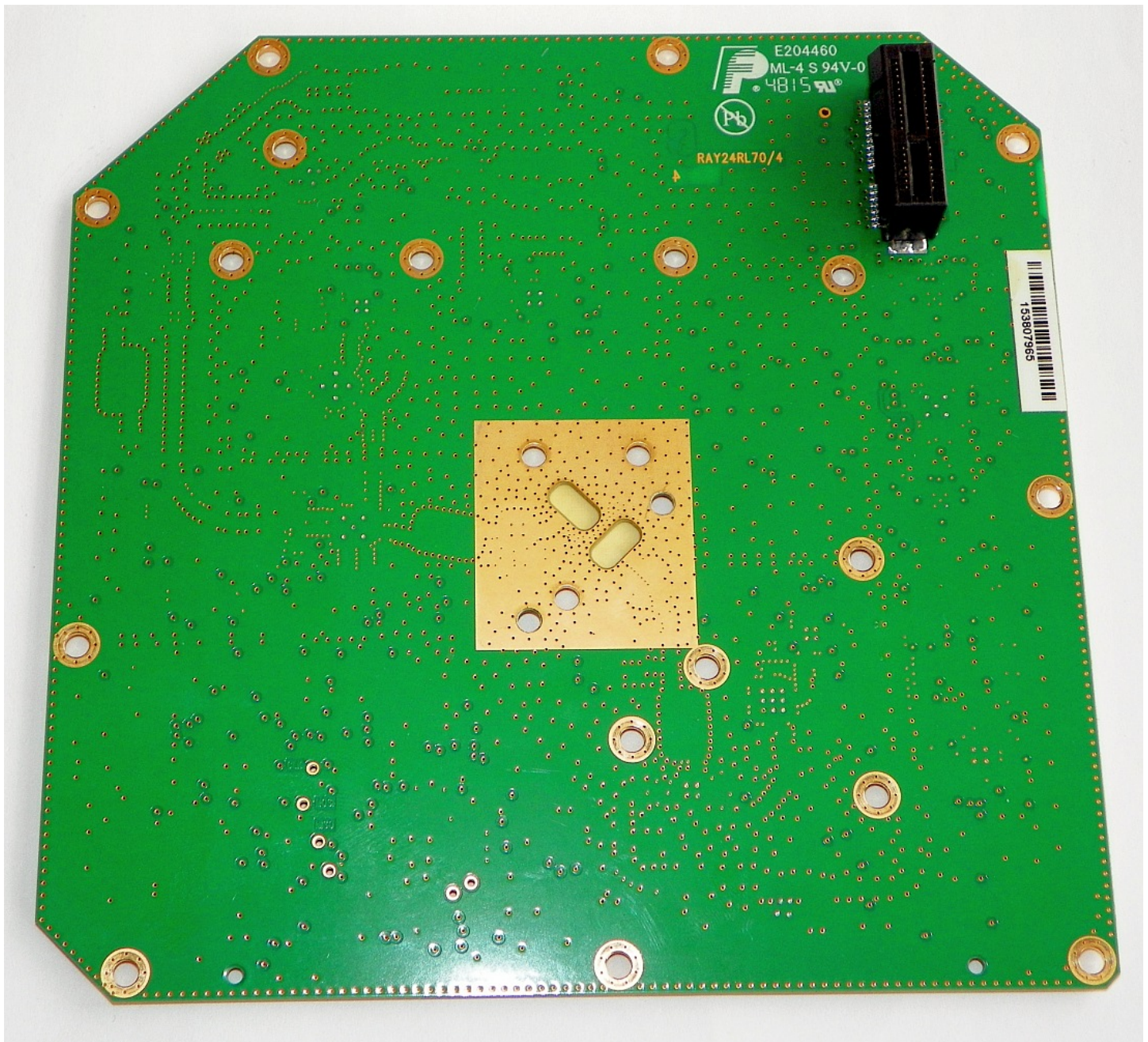
RF Board, Bottom
