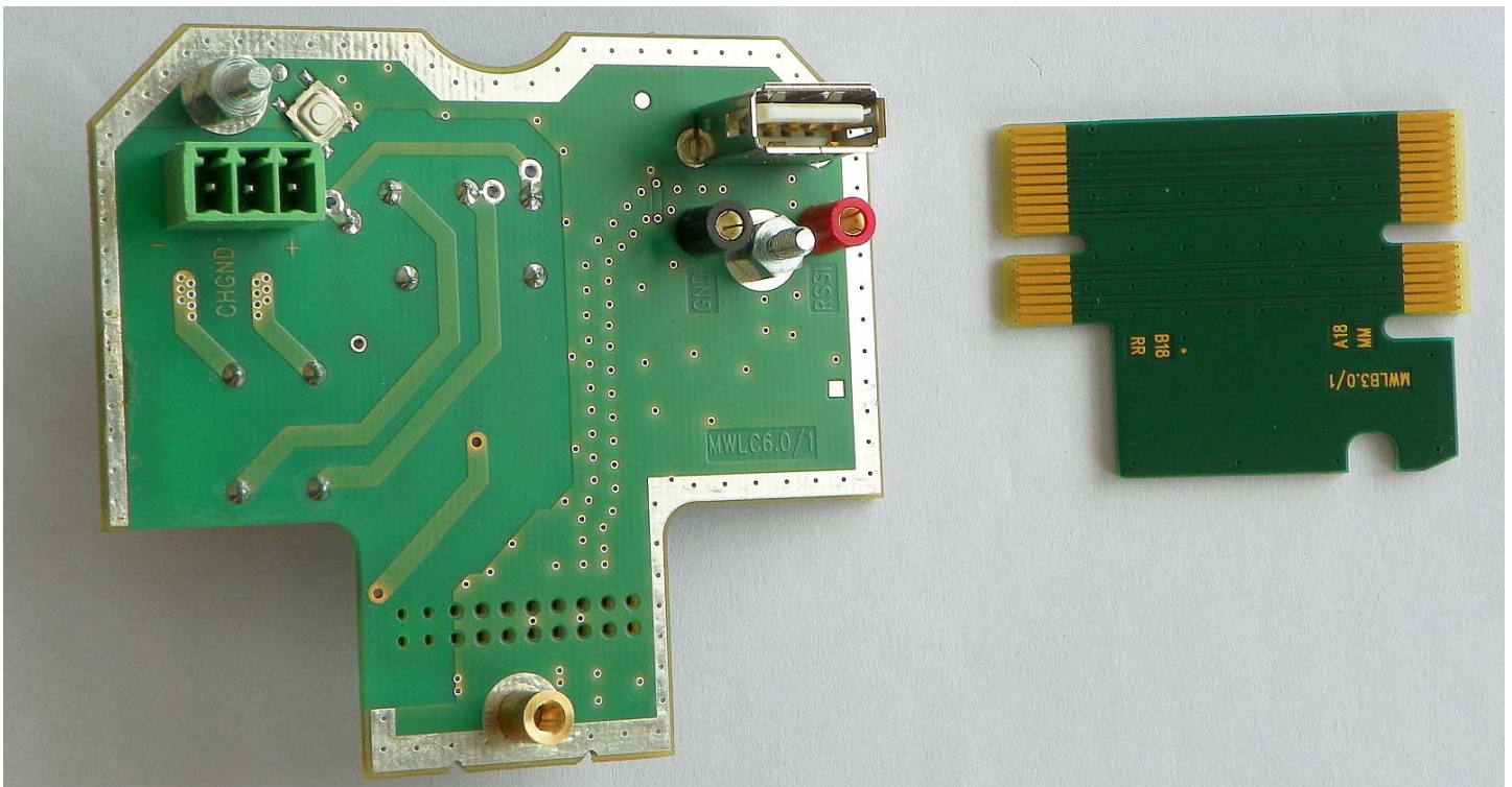
DC Power Entry &amp; USB Board, Bottom | Logic to RF Board Extender Card Side 1
