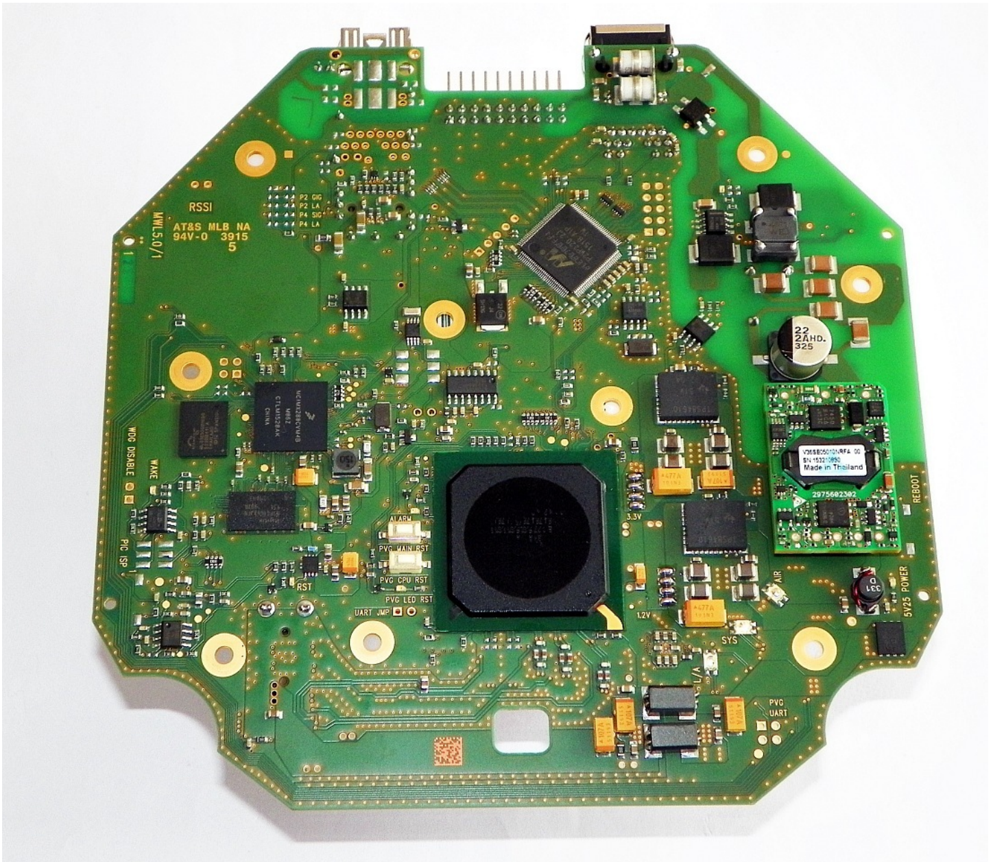
Logic Board, Top
