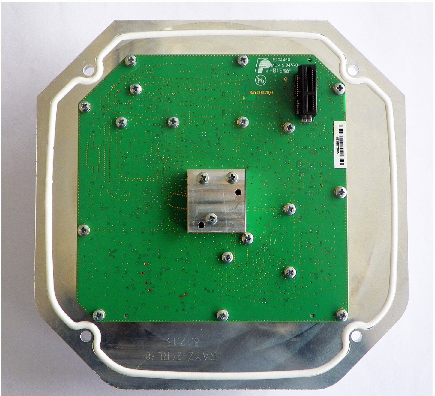
RF Board Installed To Wave Guide Assembly
