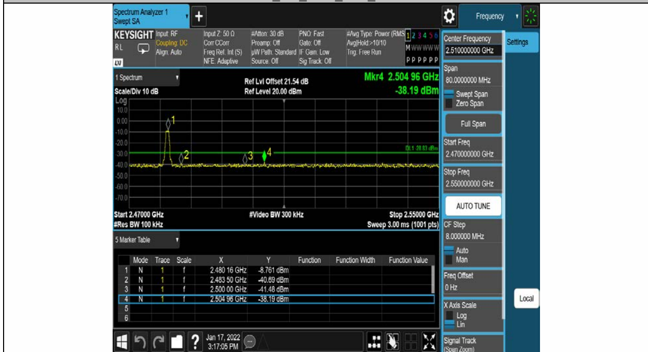
BLE_1M_Ant1_High_2480
