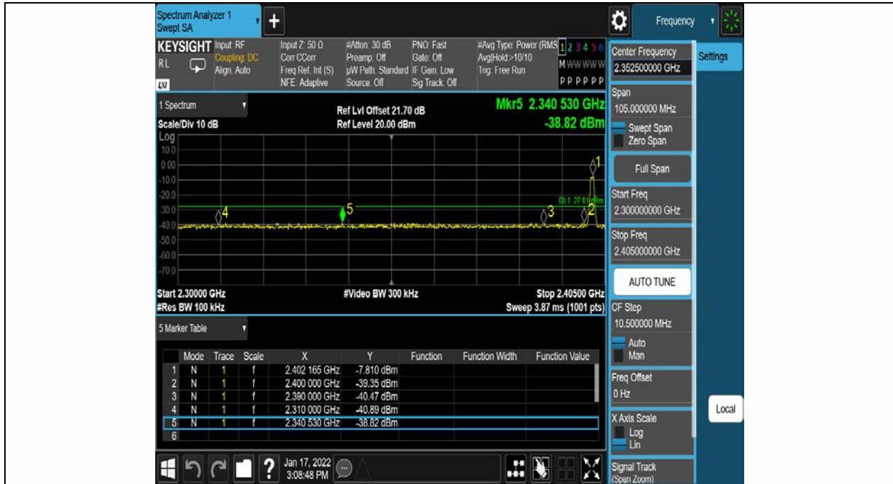
BLE_1M_Ant1_Low_2402
