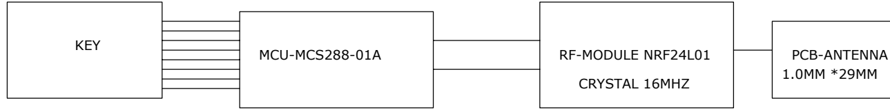
TX-BLOCK DIAGRAM
