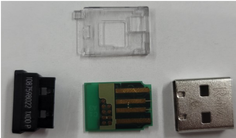
Exploded View
