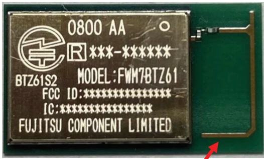
Pattern Antenna
