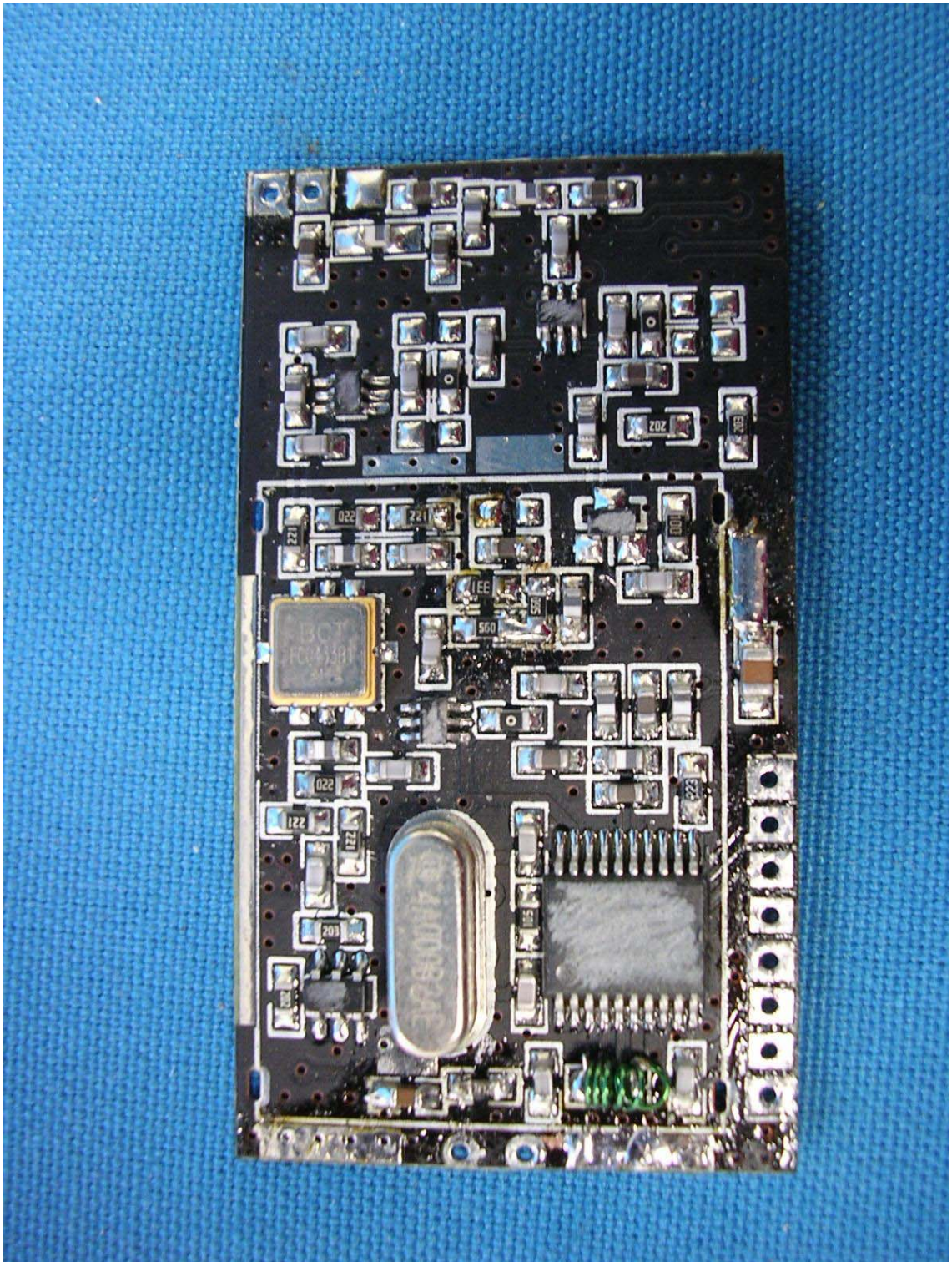
(11) EUT Photo
