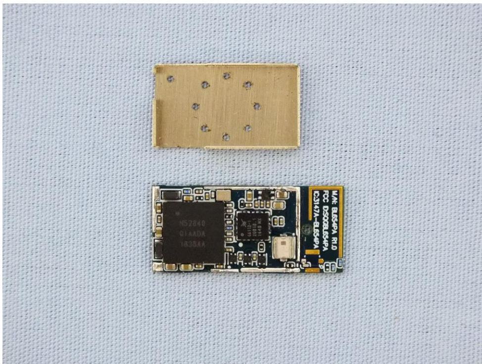
Integrated antenna
