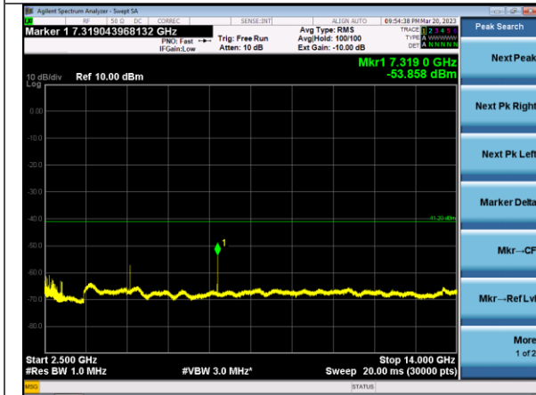
2.5-14 GHz Mid
