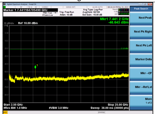
2.5-25 GHz High
