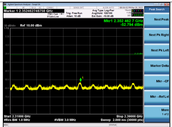
2.31-2.39 GHz High
