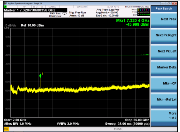
2.5-25 GHz Mid
