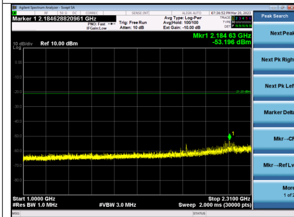
1-2.31 GHz High
