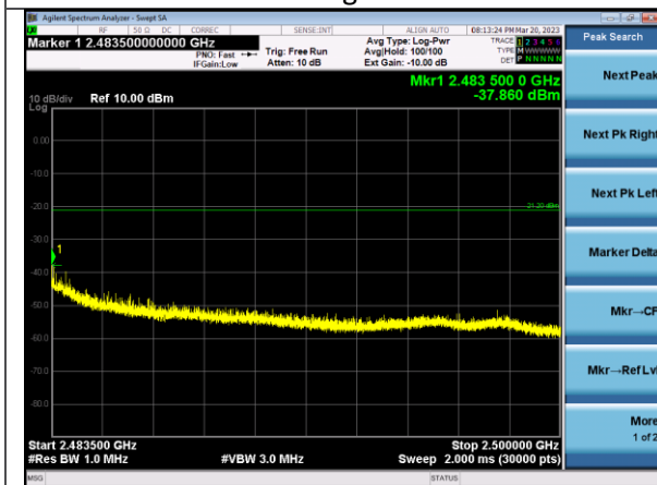
2.4835-2.5 GHz High
