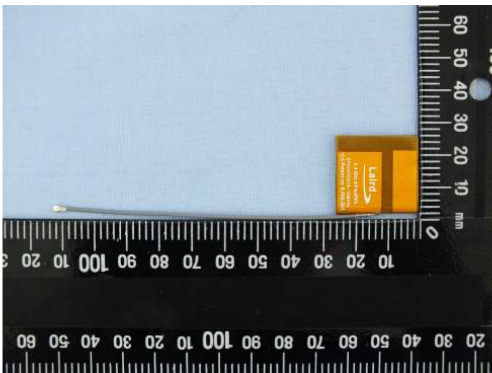
Model: mFlexPIFA
