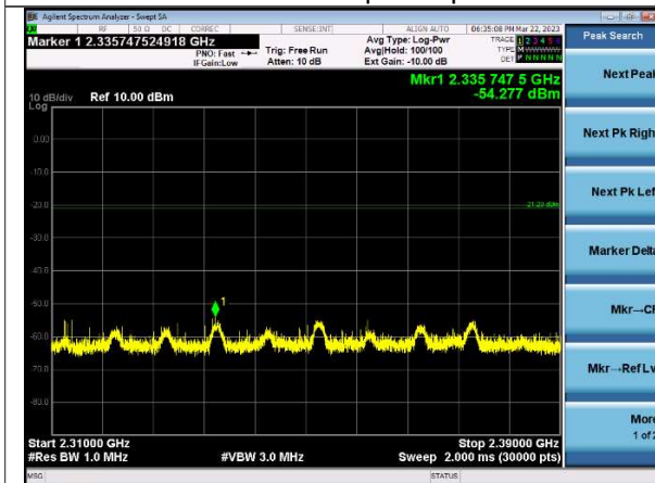
2.31-2.39 GHz Peak Channel 17 | 1 Mbps
