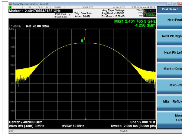
Channel 0 | 1 Mbps
