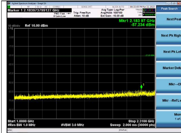
1-2.31 GHz Peak Channel 39 | 2 Mbps
