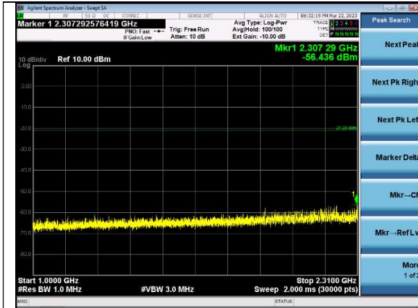
1-2.31 GHz Peak Channel 39 | 1 Mbps
