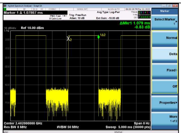
2 Mbps On Time 1.079ms
