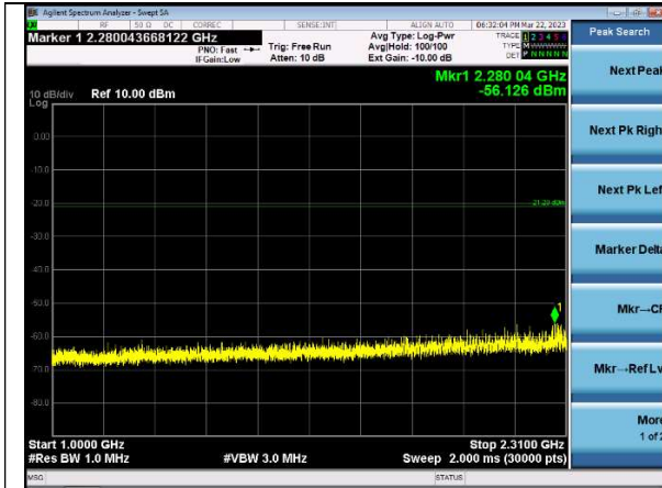
1-2.31 GHz Peak Channel 17 | 1 Mbps
