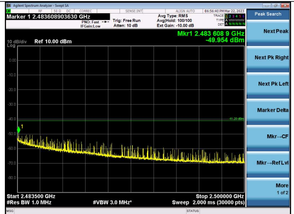
2.4835-2.5 GHz Average Channel 39 | 2 Mbps
