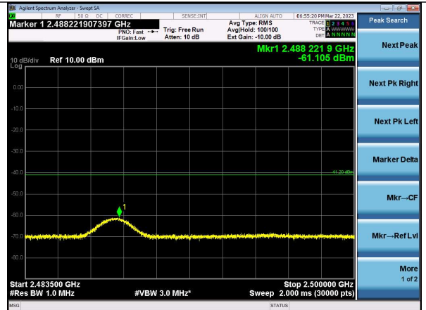
2.4835-2.5 GHz Average Channel 17 | 2 Mbps
