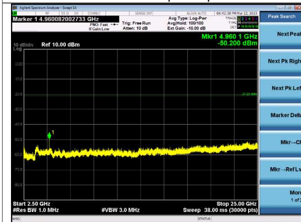
2.5-25 GHz Peak Channel 39 | 1 Mbps
