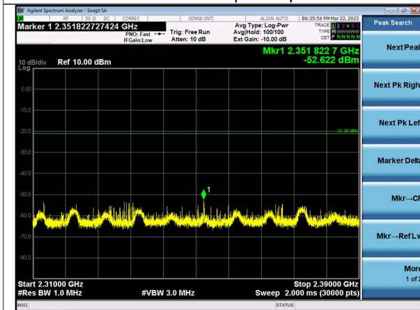
2.31-2.39 GHz Peak Channel 39 | 2 Mbps
