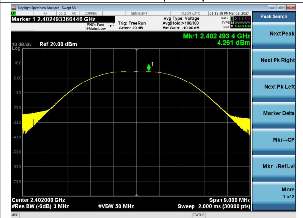
Channel 0 | 2 Mbps
