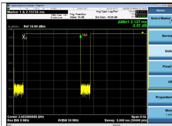
1 Mbps On Time 2.137ms
