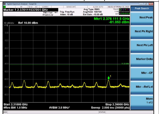
2.31-2.39 GHz Average Channel 39 | 1 Mbps
