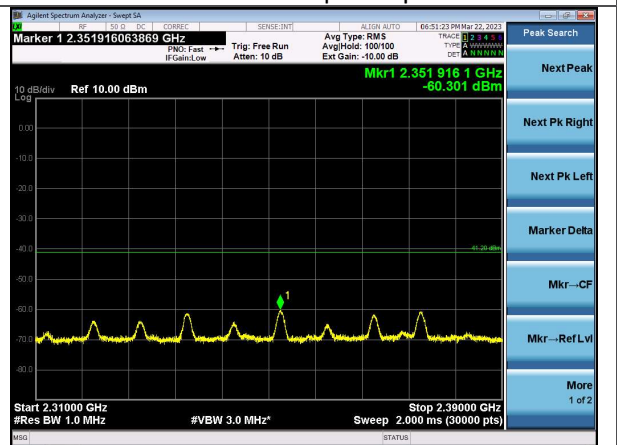
2.31-2.39 GHz Average Channel 17 | 1 Mbps
