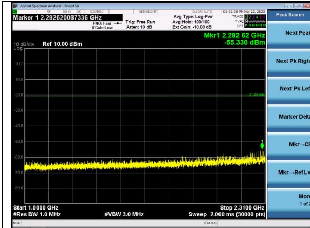
1-2.31 GHz Peak Channel 0 | 2 Mbps
