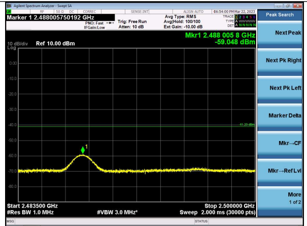
2.4835-2.5 GHz Average Channel 17 | 1 Mbps
