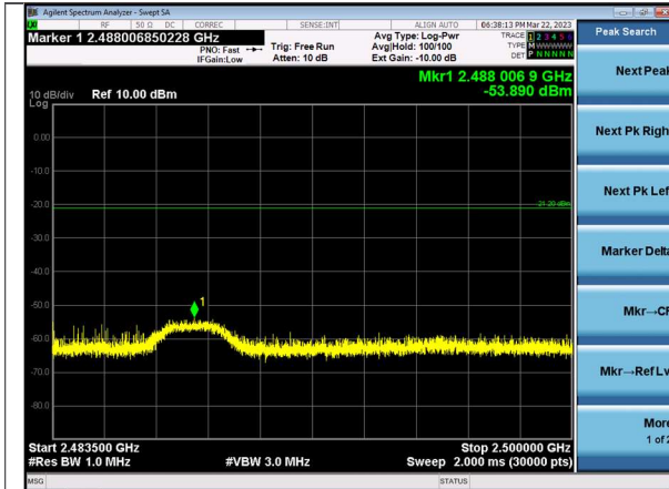
2.4835-2.5 GHz Peak Channel 17 | 2 Mbps
