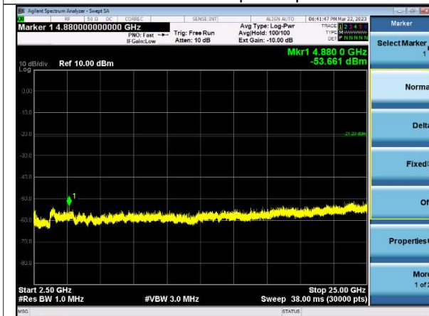
2.5-25 GHz Peak Channel 17 | 1 Mbps
