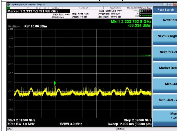
2.31-2.39 GHz Peak Channel 39 | 1 Mbps
