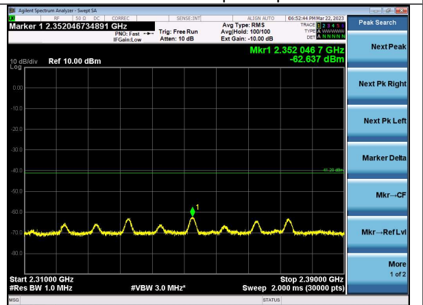
2.31-2.39 GHz Average Channel 17 | 2 Mbps
