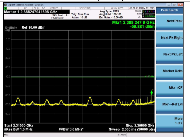
2.31-2.39 GHz Average Channel 0 | 2 Mbps
