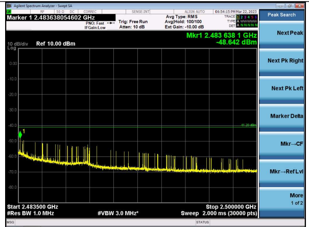
2.4835-2.5 GHz Average Channel 39 | 1 Mbps
