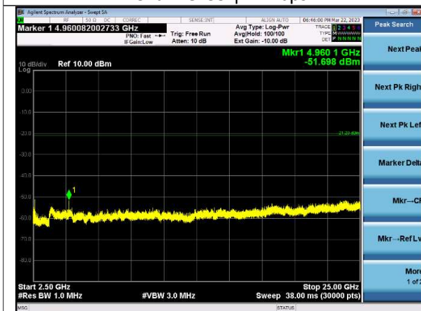
2.5-25 GHz Peak Channel 39 | 2 Mbps
