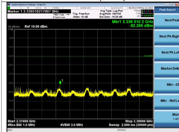
2.31-2.39 GHz Peak Channel 17 | 2 Mbps
