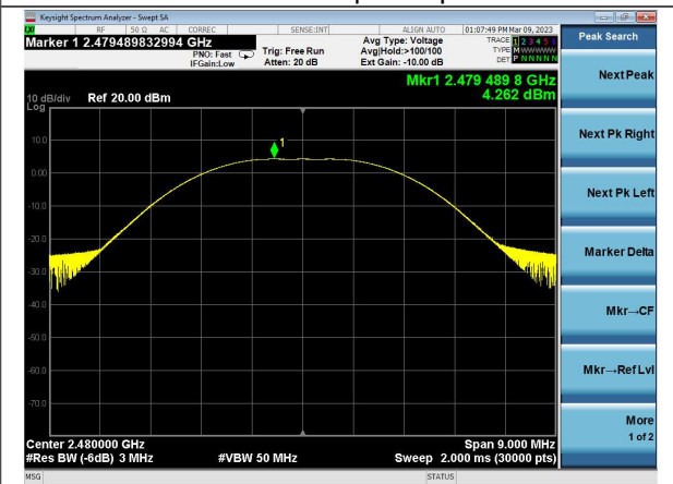
Channel 39 | 2 Mbps
