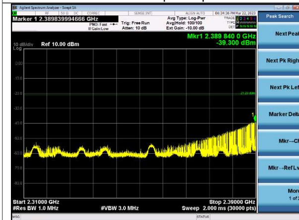
2.31-2.39 GHz Peak Channel 0 | 2 Mbps
