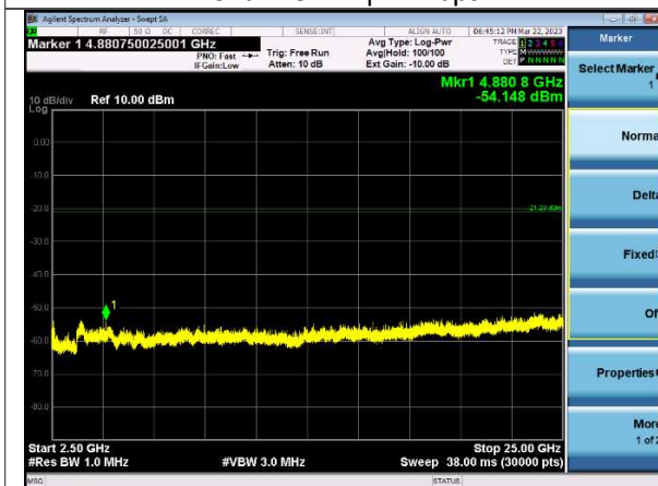
2.5-25 GHz Peak Channel 17 | 2 Mbps
