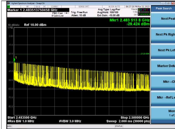
2.4835-2.5 GHz Peak Channel 39 | 1 Mbps
