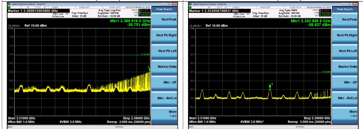
2.31-2.39 GHz Peak Channel 0 | 1 Mbps
