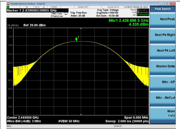
Channel 17 | 1 Mbps
