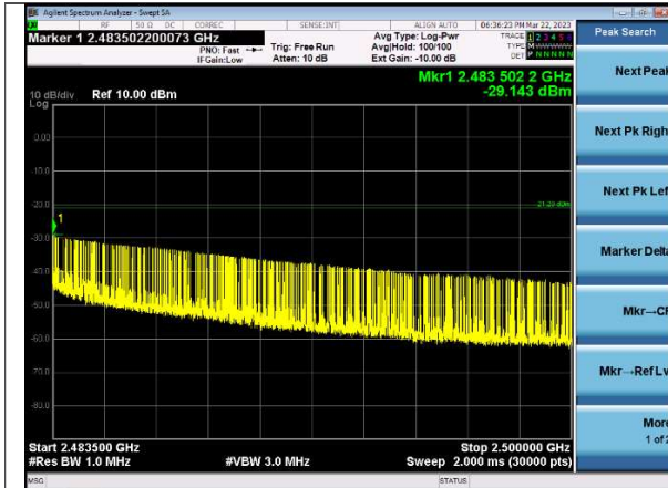
2.4835-2.5 GHz Peak Channel 39 | 2 Mbps
