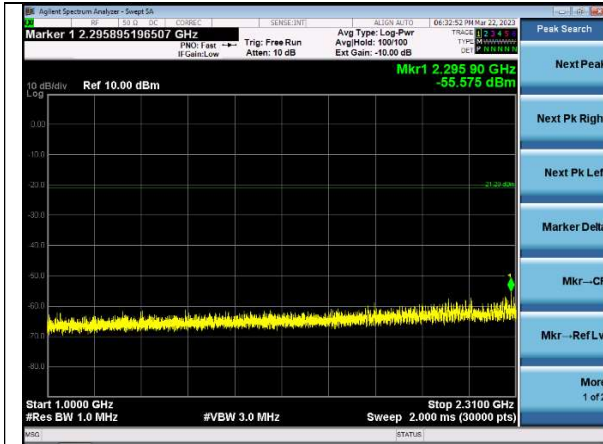
1-2.31 GHz Peak Channel 17 | 2 Mbps
