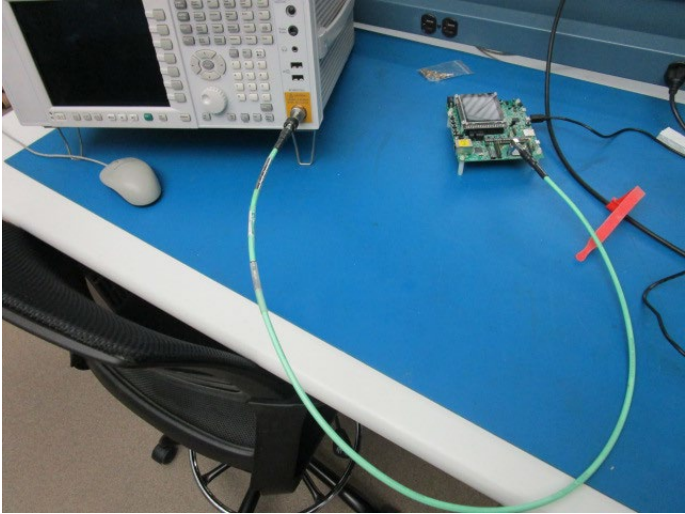
Conducted Measurements
