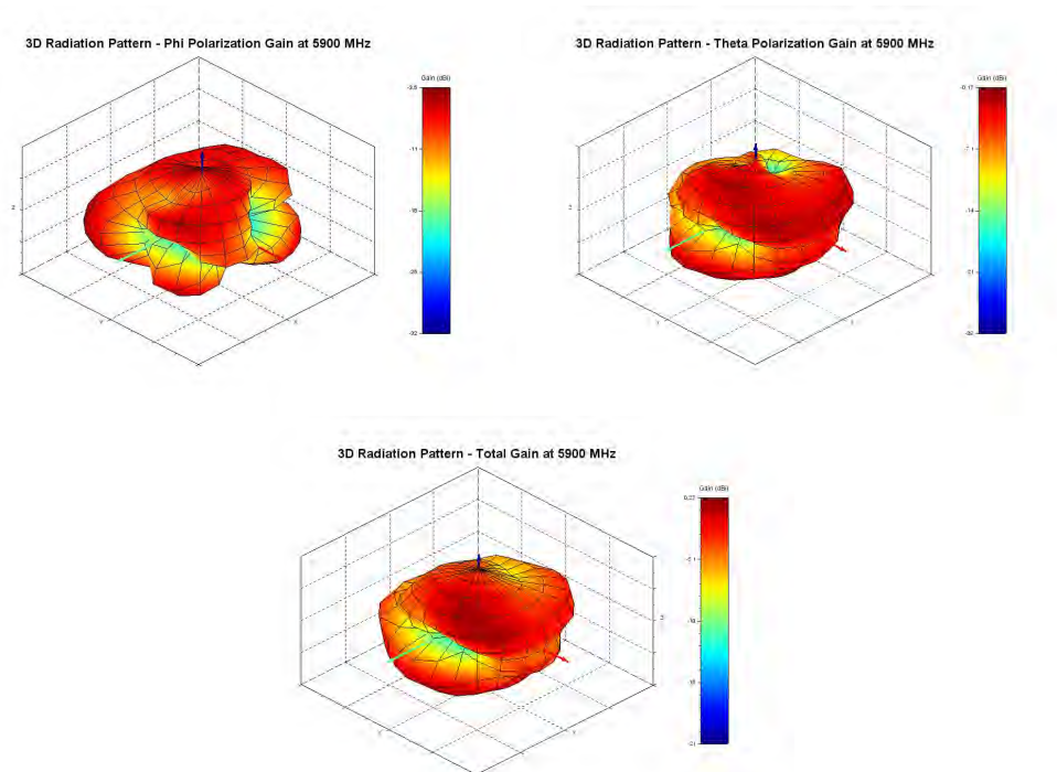
Figure 11: Phi, Theta, and total gain plots
