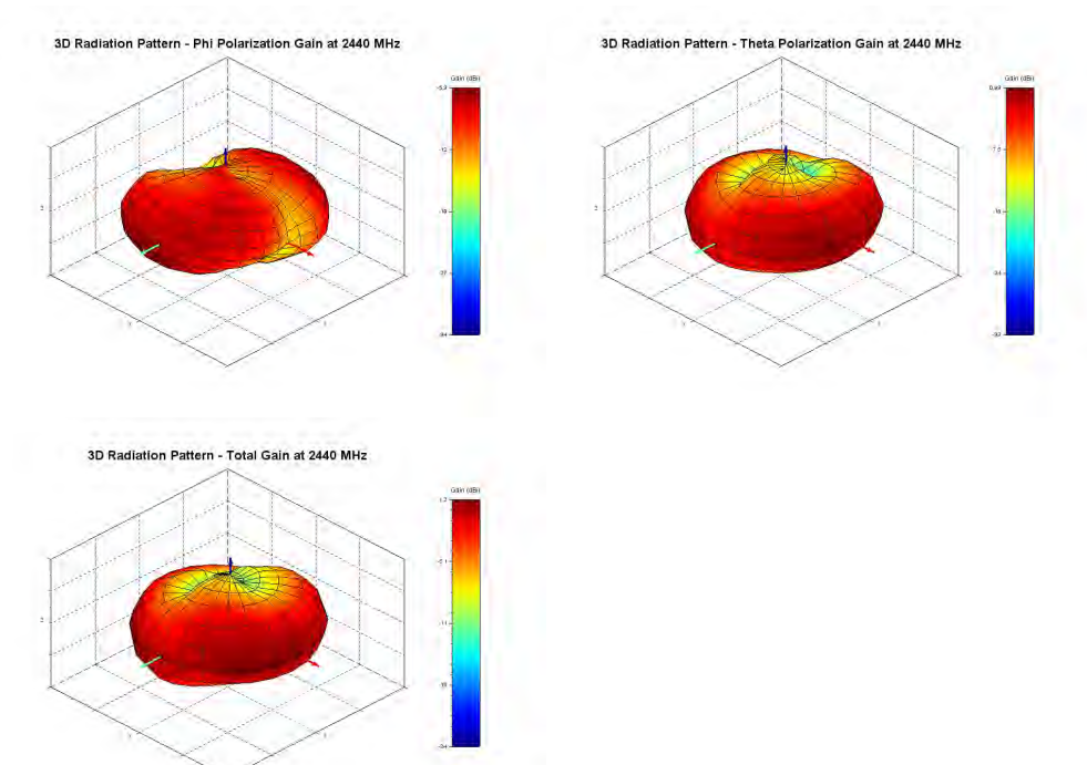
Figure 5: Phi, Theta, and total gain plots
