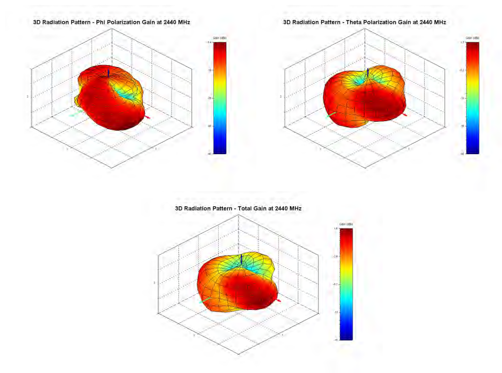
Figure 23: Phi, Theta, and total gain plots
