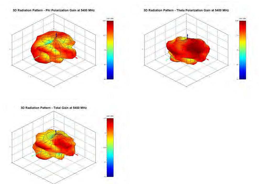
Figure 27: Phi, Theta, and total gain plots
