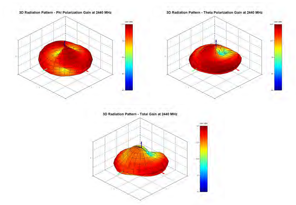
Figure 14: Phi, Theta, and total gain plots
