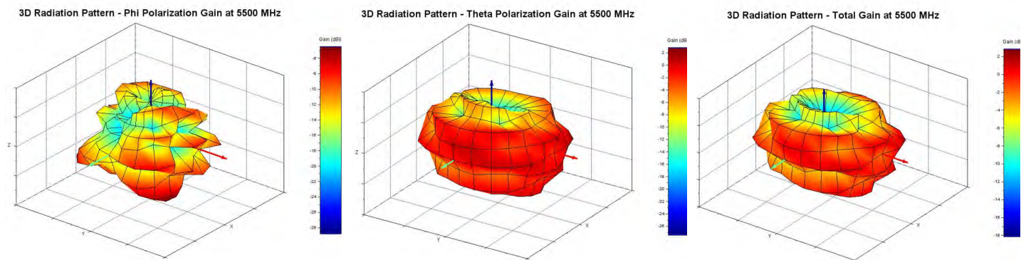
Figure 9: Phi polarization, Theta polarization and, and total gain plots – 5500 MHz
