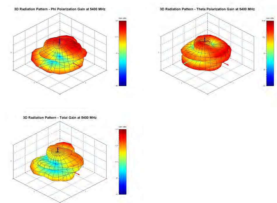
Figure 18: Phi, Theta, and total gain plots
