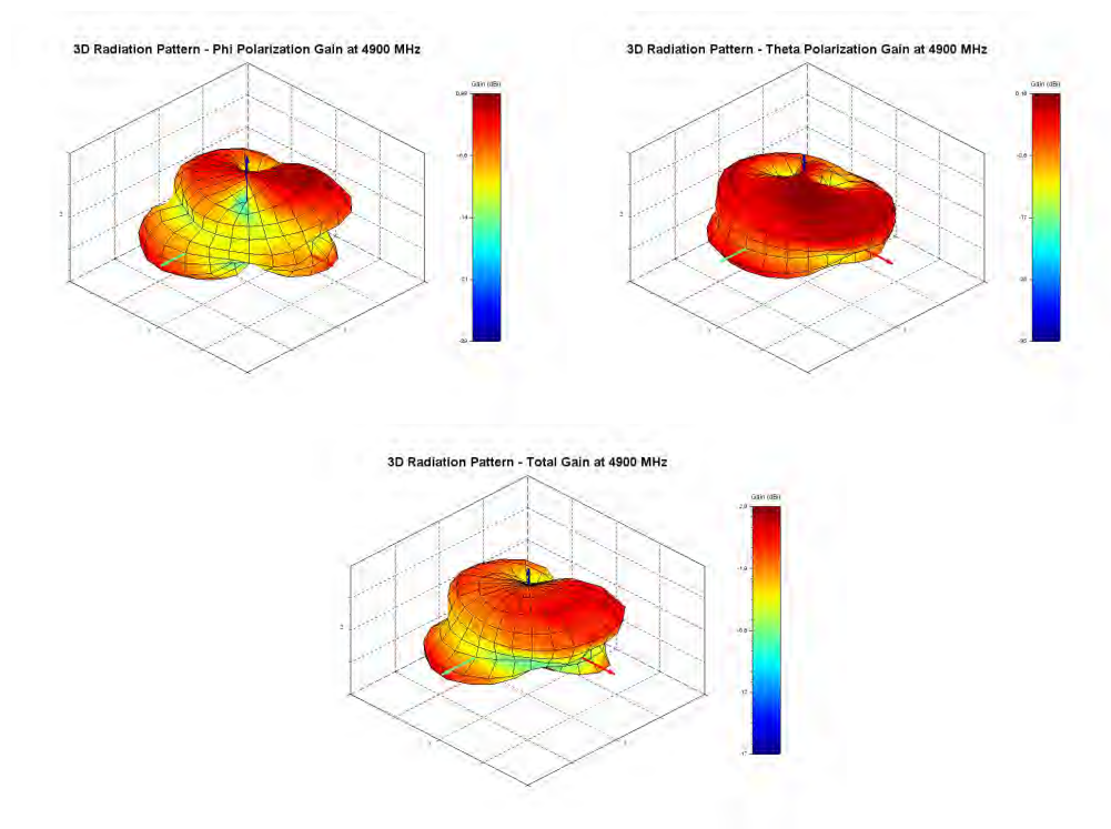
Figure 16: Phi, Theta, and total gain plots
