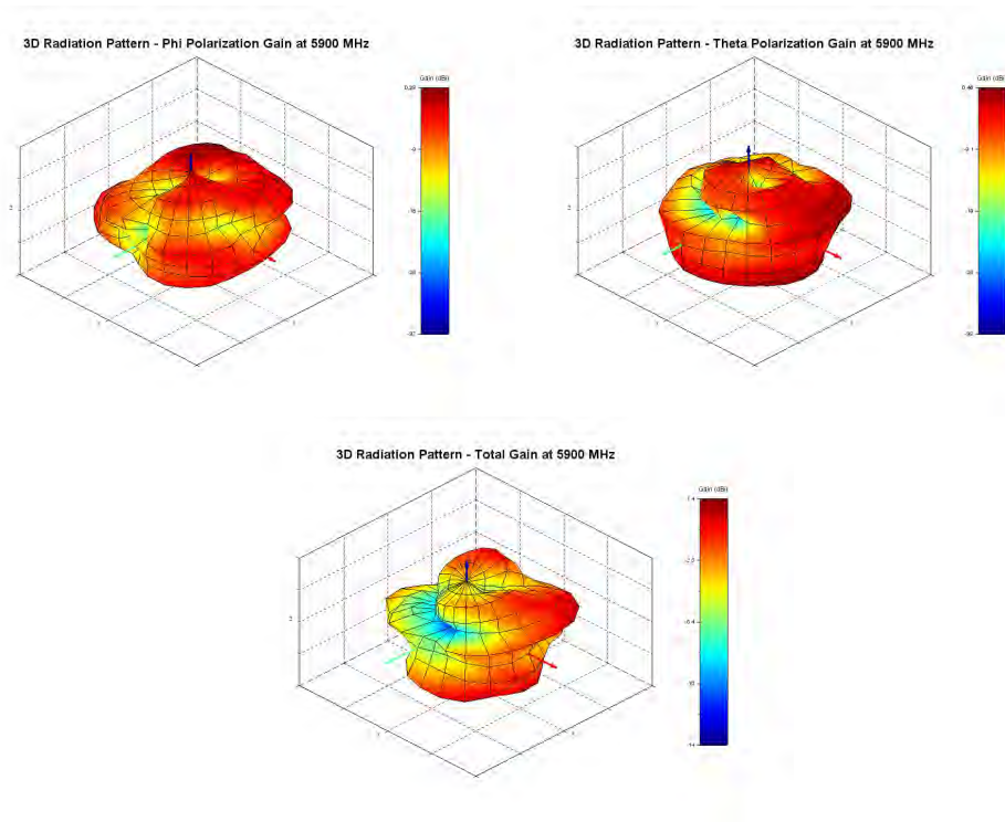
Figure 20: Phi, Theta, and total gain plots
