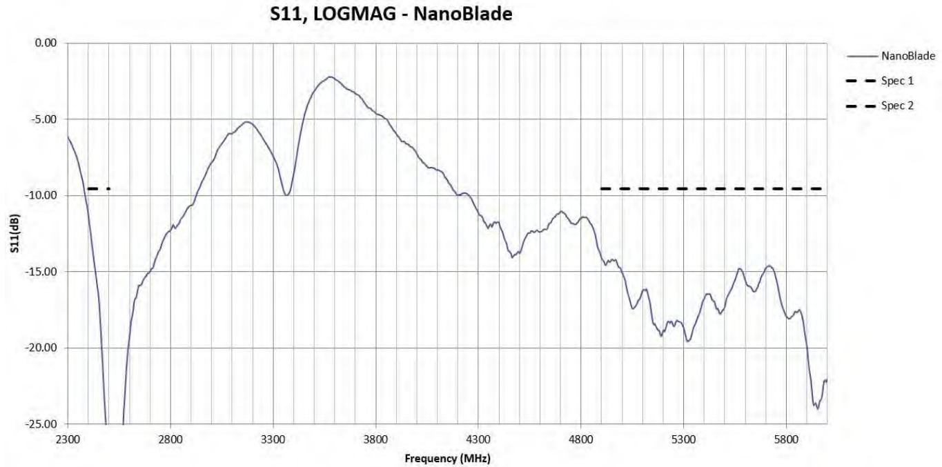
Figure 2: Antenna Return Loss measured in free space
