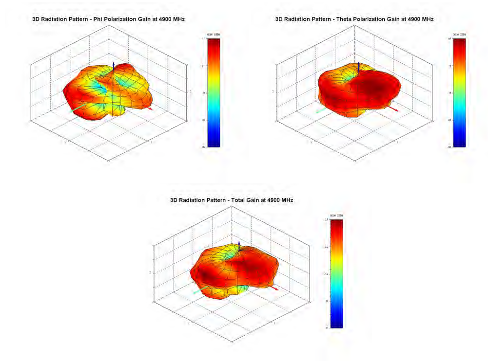
Figure 25: Phi, Theta, and total gain plots
