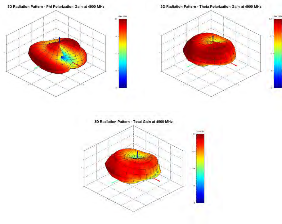
Figure 7: Phi, Theta, and total gain plots
