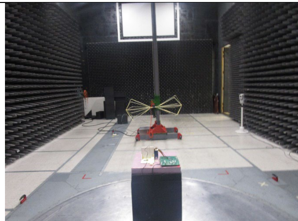
30-200 MHz Radiated
