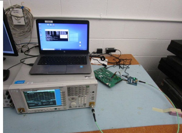
RF Conducted
