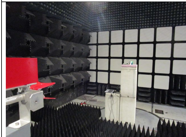
25-40GHz Radiated
