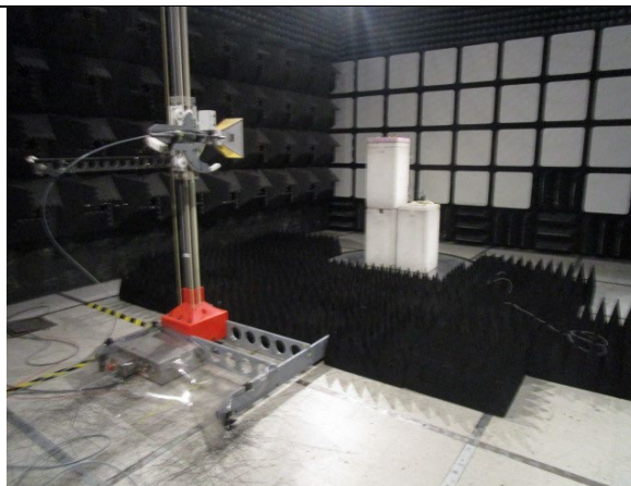
1-4 GHz Radiated
