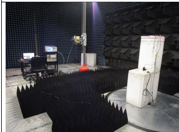
4-18GHz Radiated
