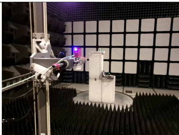
18-25GHz Radiated
