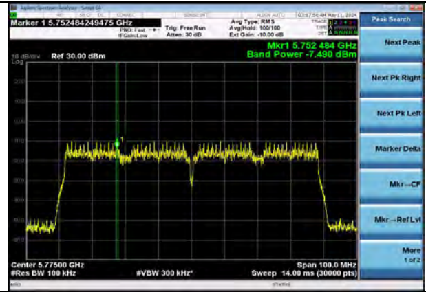
802.11ac80 | Channel 155 | MCS9
