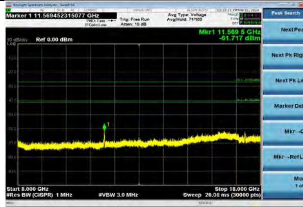
802.11a | Channel 157 | 6 Mbps | 8000-18000 MHz
