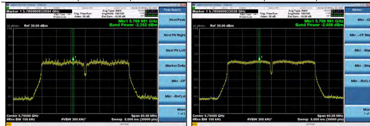
802.11n40 | Channel 159 | MCS7
