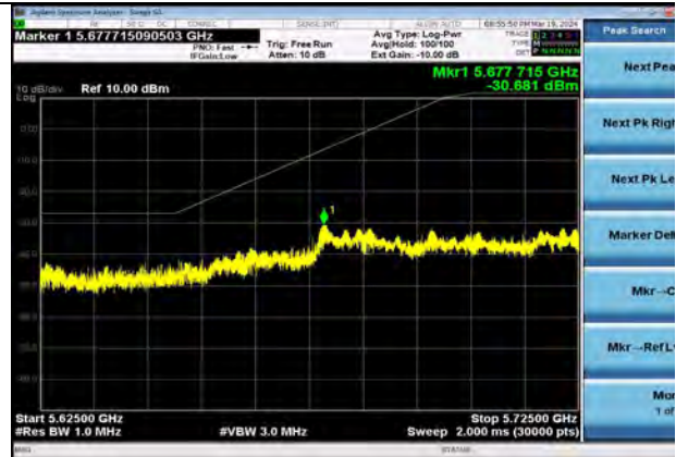
802.11ac80 | Channel 155 | MCS7
