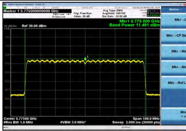
802.11ax80 | Channel 155 | MCS0
