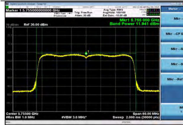
802.11ax40 | Channel 151 | MCS0
