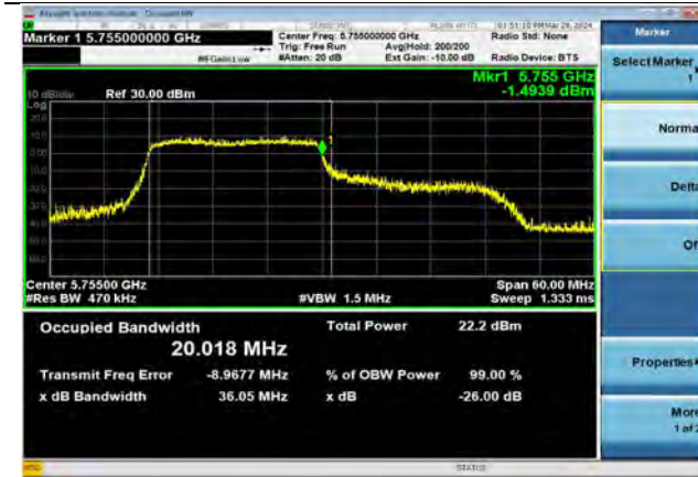
802.11ax40 | Channel 151 | MCS0 | RU Tone 242 Index 61
