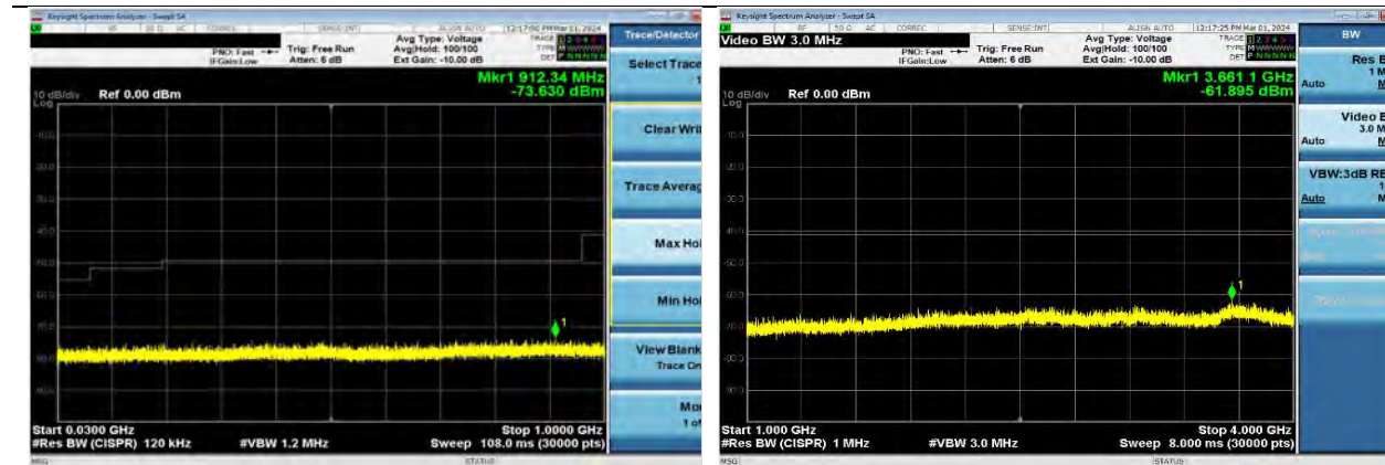
802.11a | Channel 149 | 6 Mbps | 30-1000 MHz 802.11a | Channel 149 | 6 Mbps | 1000-4000 MHz
