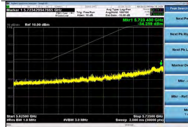
802.11ax40 | Channel 151 | MCS9
