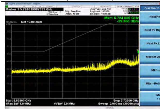
802.11ax40 | Channel 151 | MCS0 | RU106
