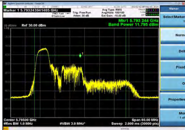
802.11ax40 | Channel 159 | MCS0 | RU 52
