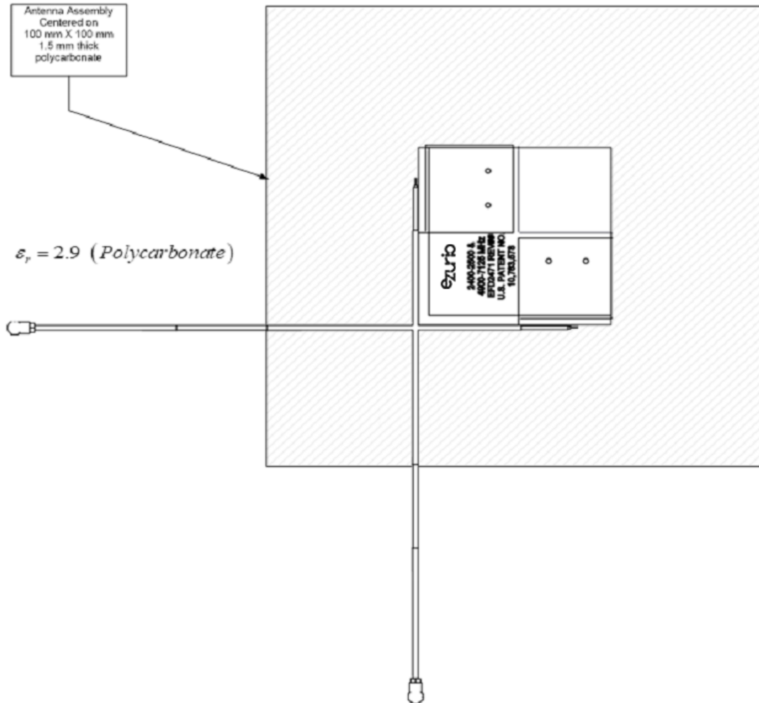
Figure 1: Nominal placement of FlexPIFA MIMO Antenna array on 100 mm X 100 mm, 1.5 mm thick, polycarbonate sheet
