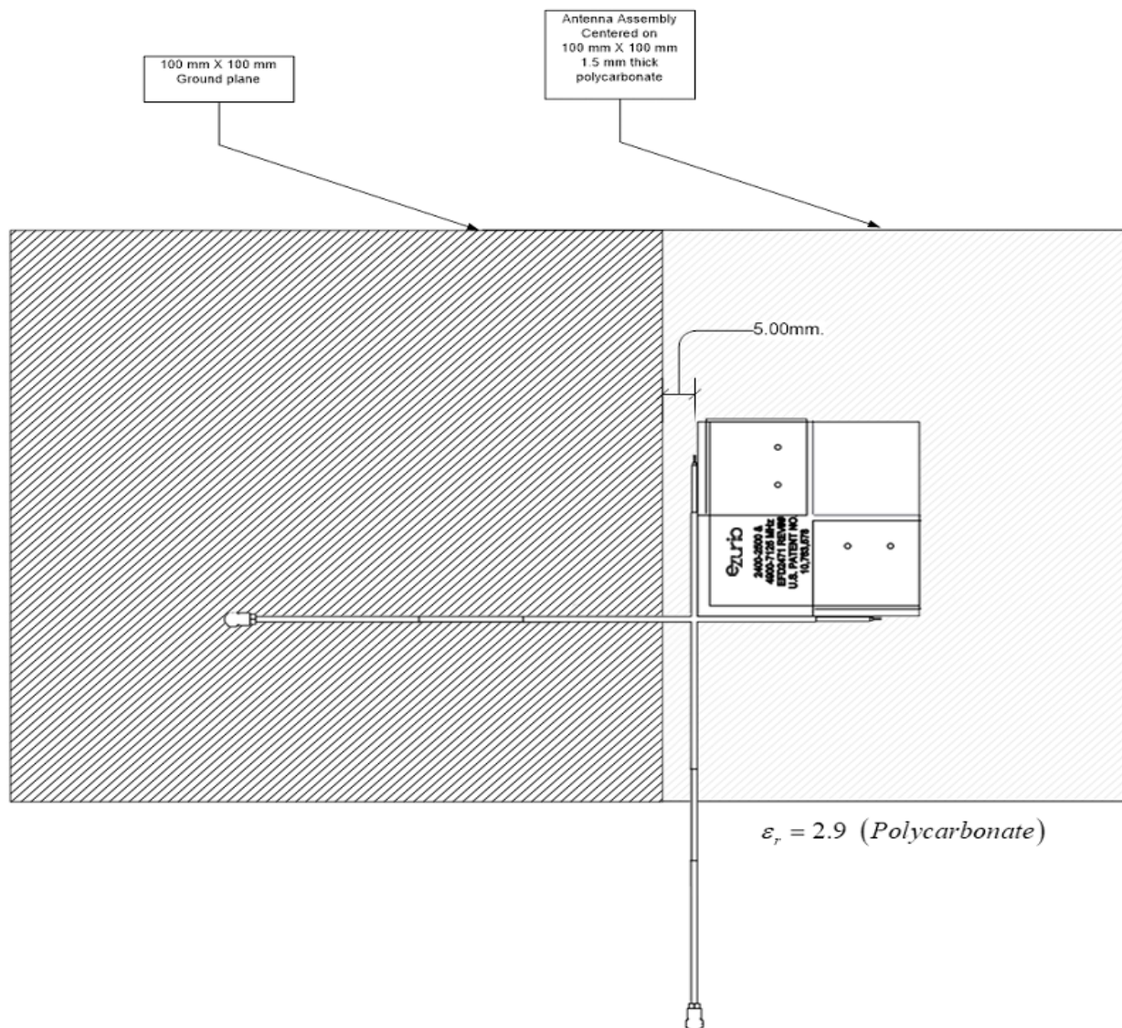
Figure 2: Minimum clearance between co-planar edge-coupled ground planes for one placement instance
