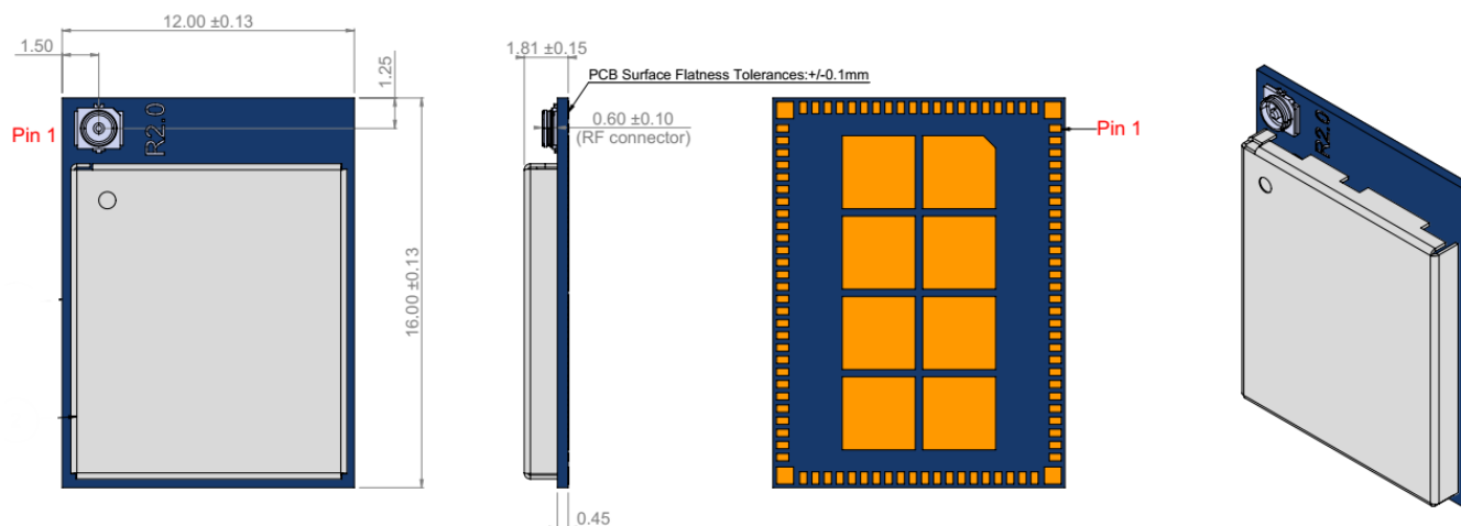
Figure 16: M.2 1216 (MHF4 variant) Non-Antenna Diversity type
