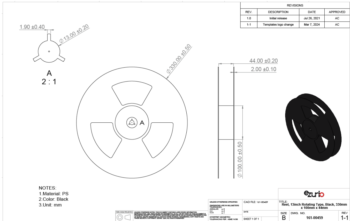
Figure 23: Sona IF513 Reel specifications, 161-00459
