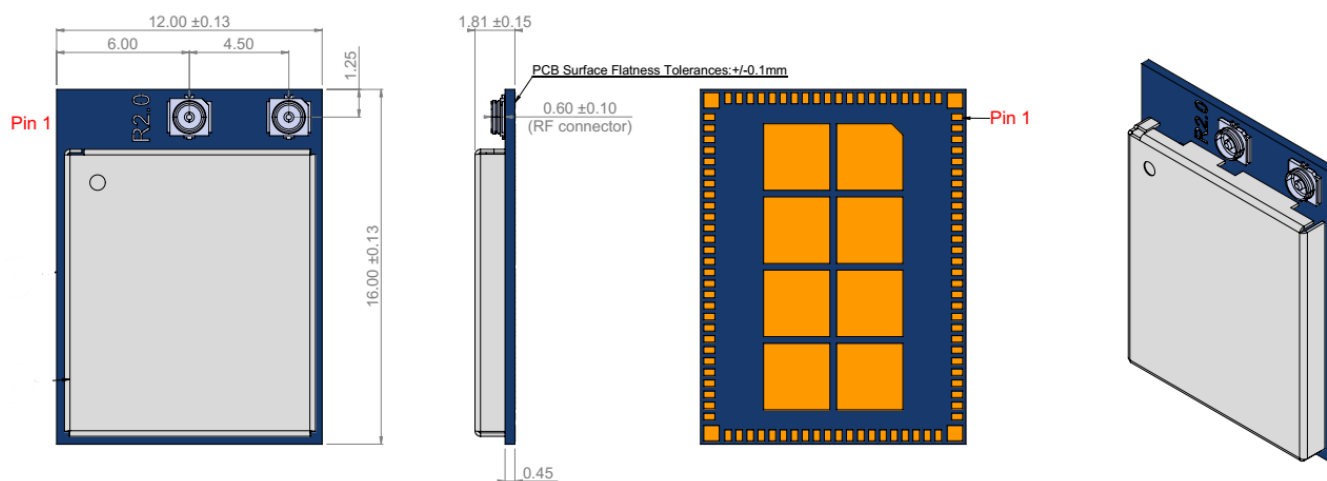
Figure 18: M.2 1216 (MHF4 variant) Antenna Diversity type
