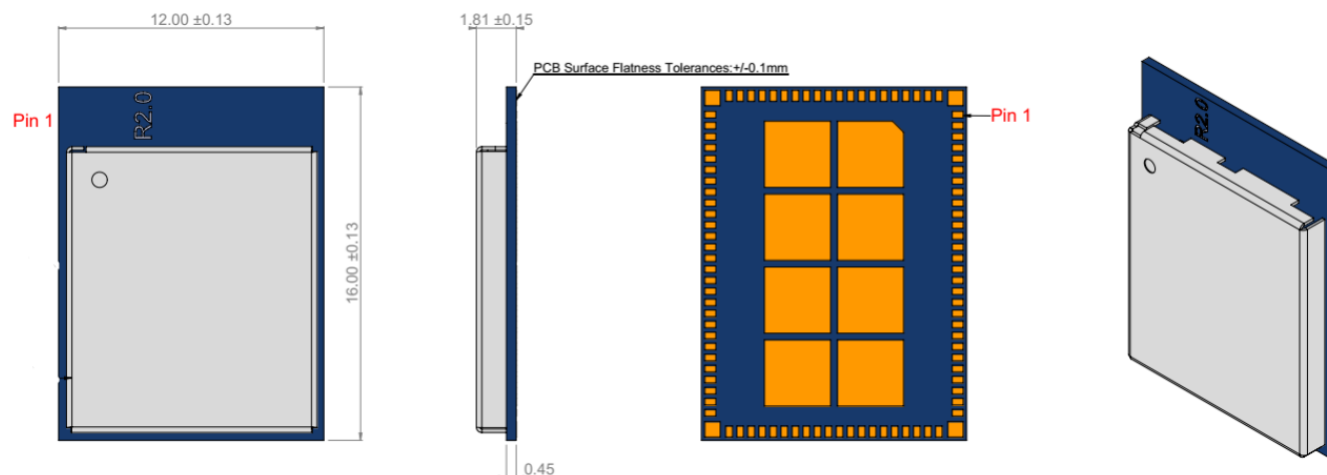
Figure 17: M.2 1216 (Trace variant) Non-Antenna Diversity type
