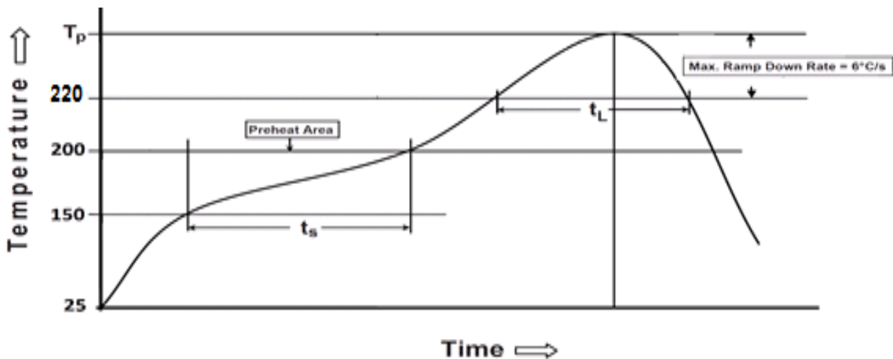
Figure 35: Temperature profile
