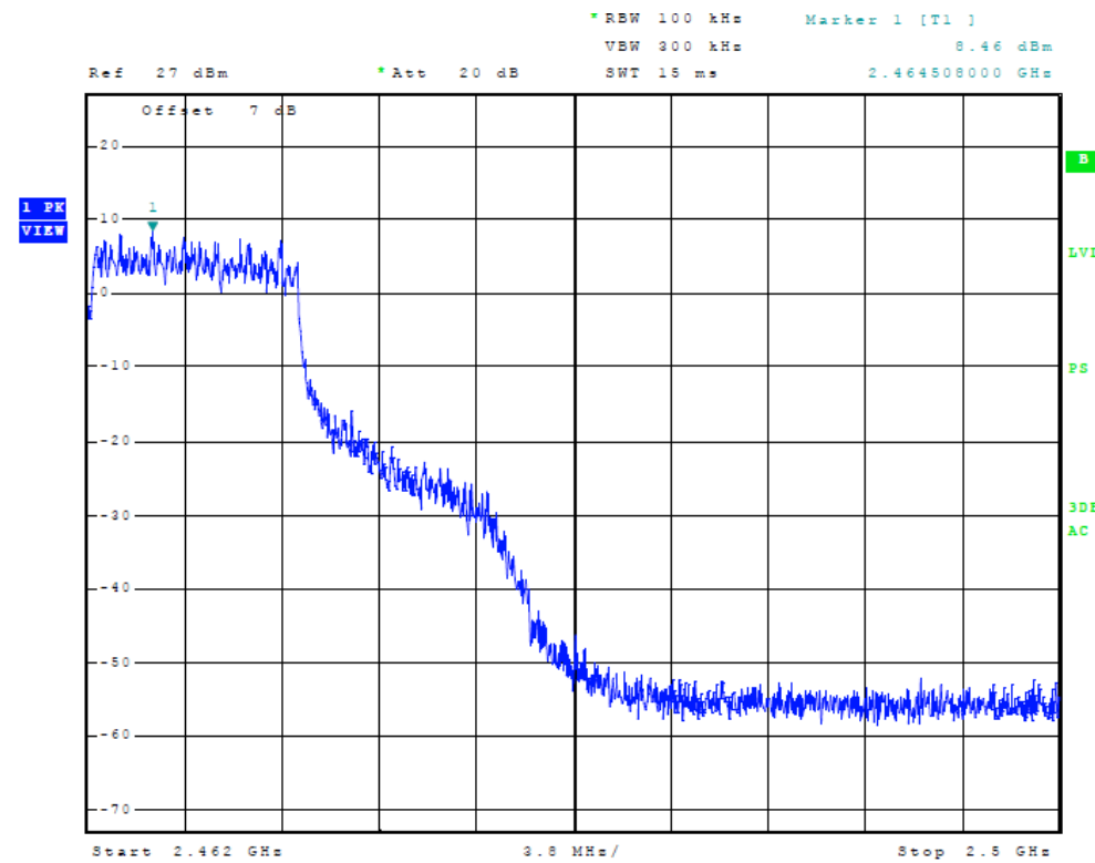
Figure 10 Plot of Transmitter High Band Edge (802.11 g-mode)
