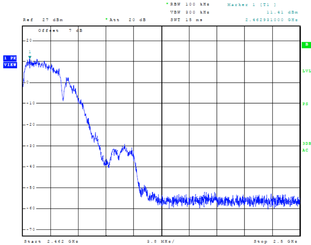
Figure 9 Plot of Transmitter High Band Edge (802.11 b-mode)
