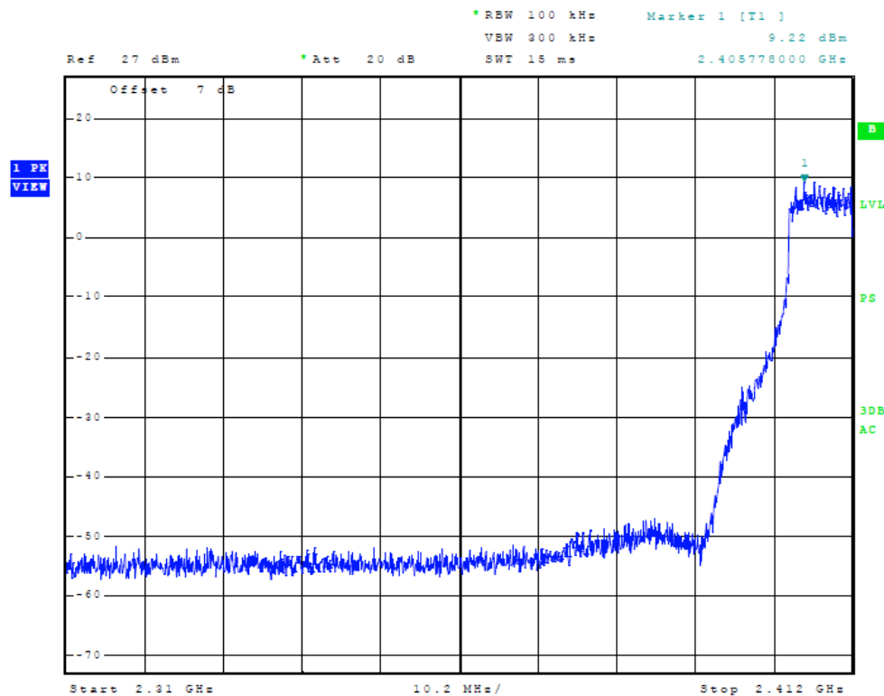
Figure 8 Plot of Transmitter Low Band Edge (802.11 g-mode)
