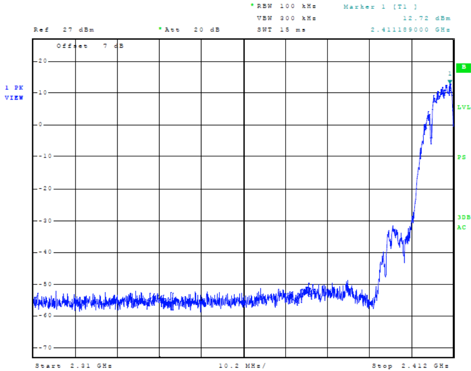
Figure 7 Plot of Transmitter Emissions Low Band Edge (802.11 b-mode)
