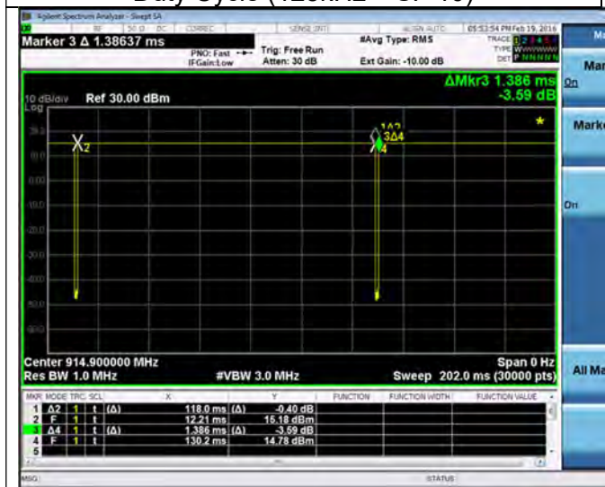
Duty Cycle (125 kHz – SF 7)
