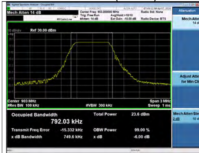
6dB bandwidth (Low)
