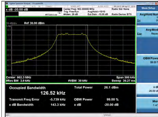
Occupied/20dB bandwidth (Low)
