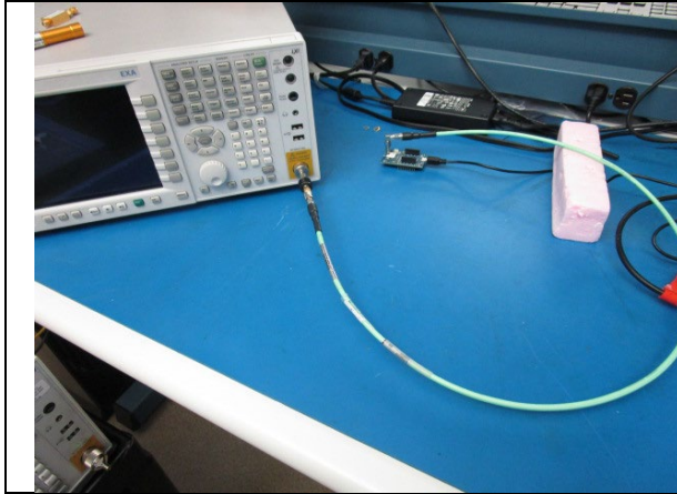
Conducted Setup
