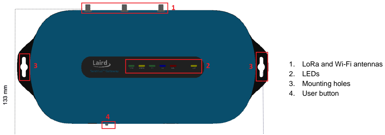
Figure 1: Top of the Sentrius™ RG191+LTE gateway
