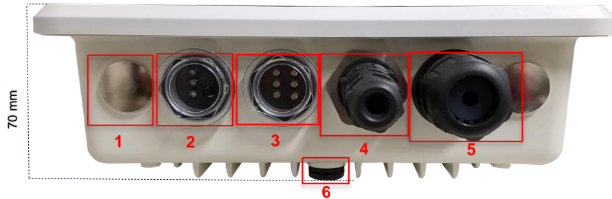
Figure 50: Side panel of the IP67 Rated Sentrius™ RG191+LTE Gateway (Revision 1 & 2)
