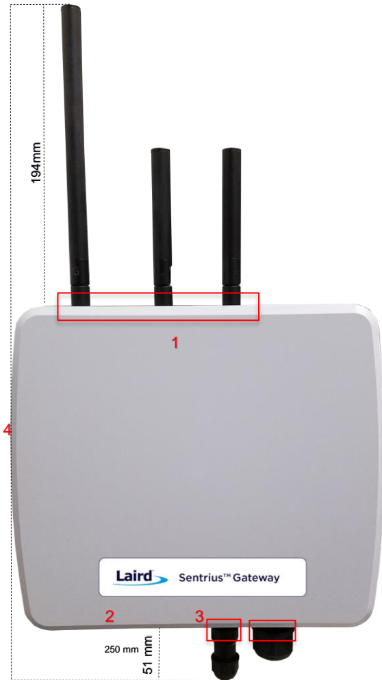
Figure 46: Top of the IP67 Rated Sentrius™ RG191+LTE Gateway
