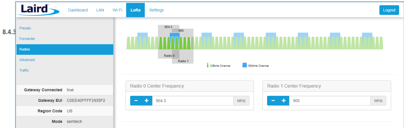
Figure 28: Channel assignments
