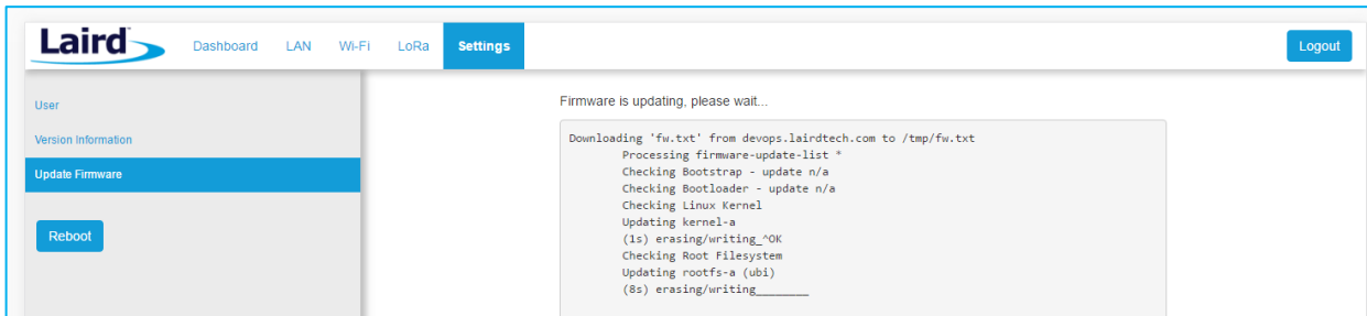
Figure 40: Progress indicator
