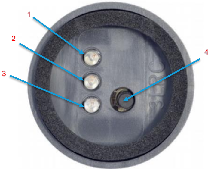
Figure 48: LED displays with User button (#6 from Figure 47)
