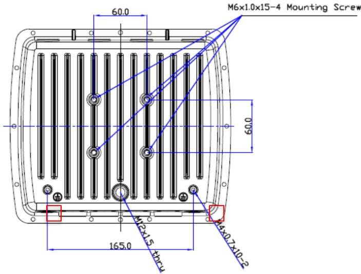
Figure 59: Enclosure placement dimensions (mm)
