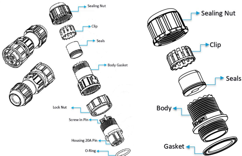
Figure 51: Power cable (left) and Ethernet (right) assembly components
