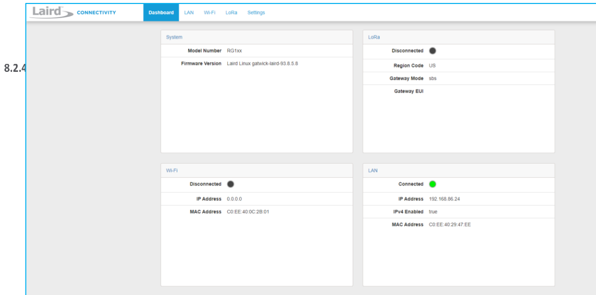
Figure 25: Dashboard view
