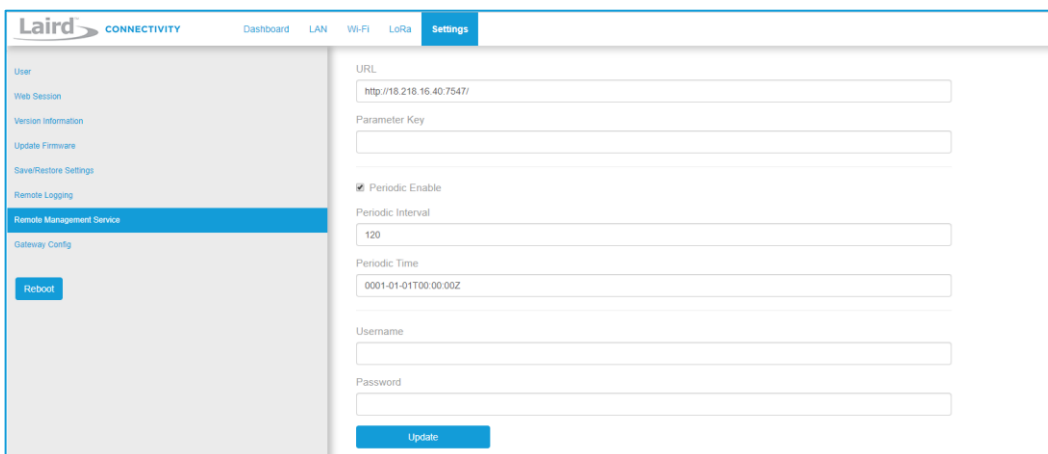
Figure 43: Save/Restore settings
