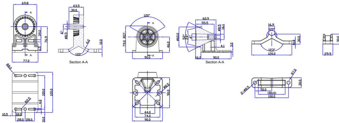
Figure 61: Pole mount dimensions
