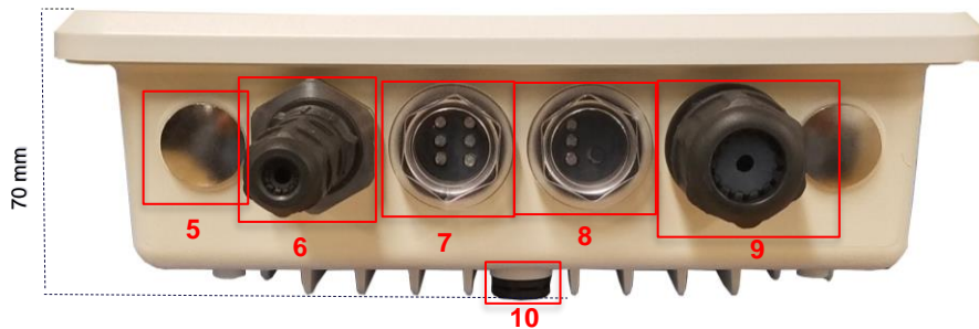
Figure 47: Side panel of the IP67 Rated Sentrius™ RG191+LTE Gateway (Current Generation)
