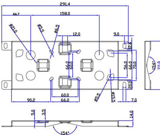
Figure 58: Wall mount dimensions
