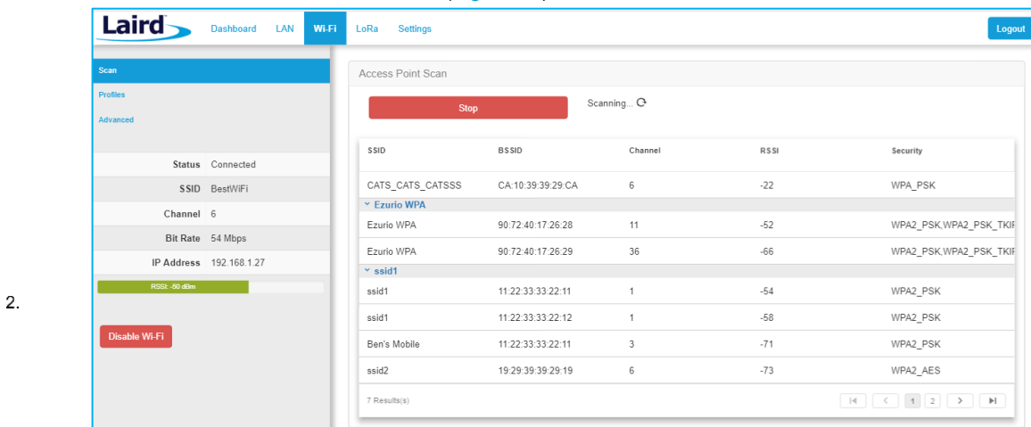
Figure 14: Scan function
