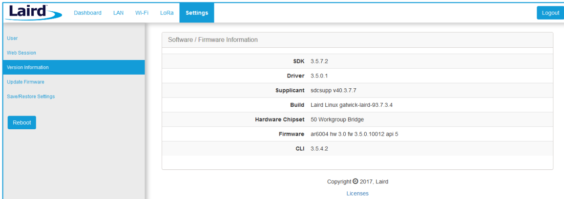
Figure 38: Version information
