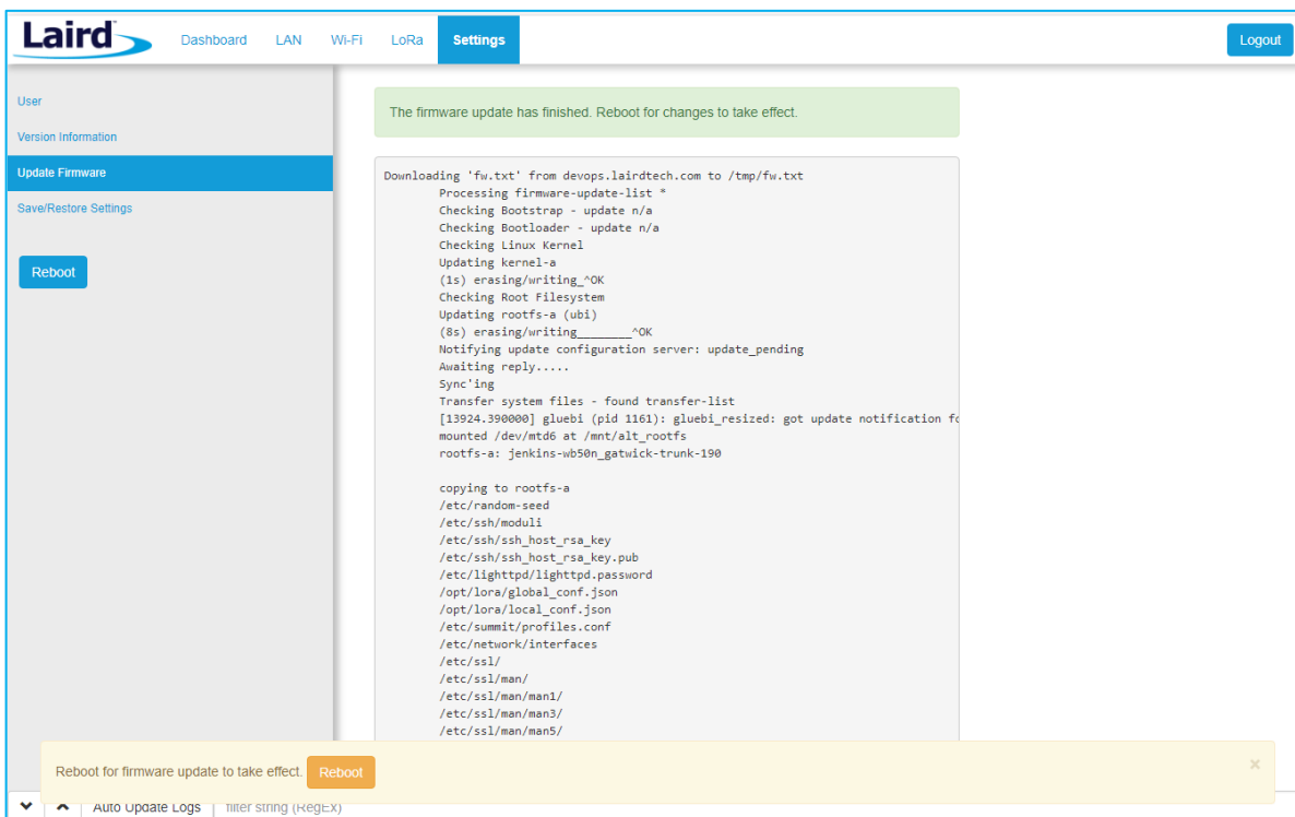
Figure 41: Reboot prompt
