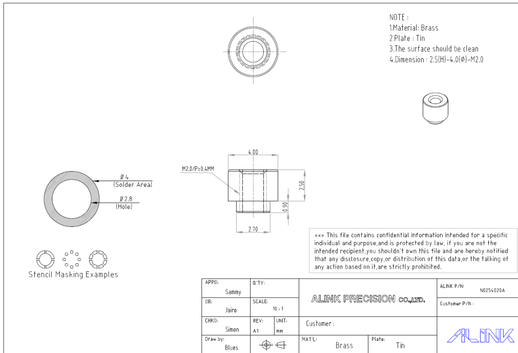
Figure 9: PEM Threaded Standoff mechanical drawings
