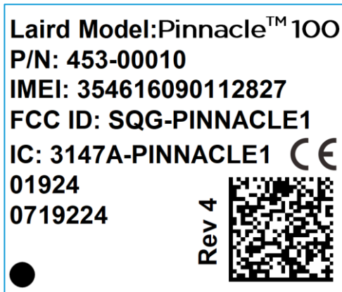
Figure 13: 453-00010 modem label
