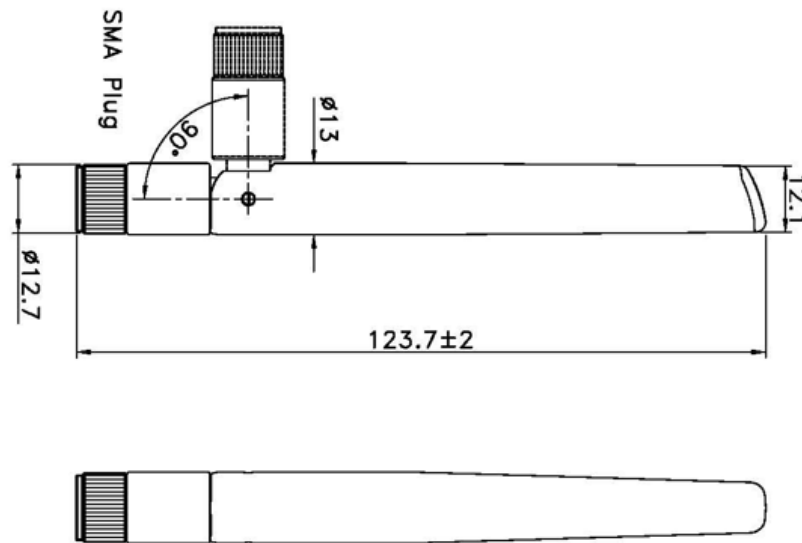
Figure 2. Antenna Dimensions
