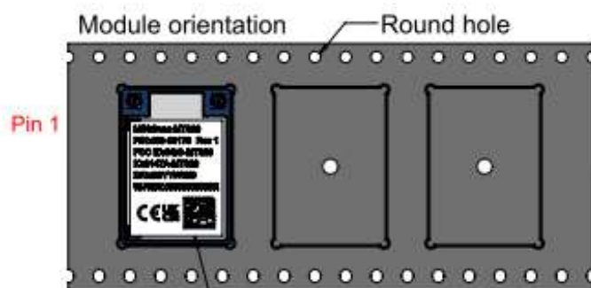
Figure 9: Module Orientation in Carrier Tape Pocket, MHF4 Variant
