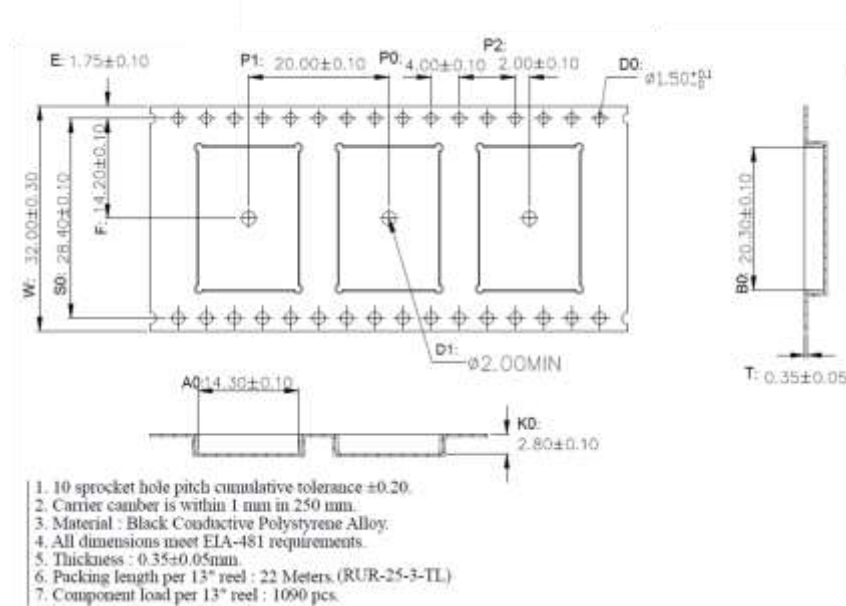
Figure 7: Sona MT320 M.2 1420 Tape specifications
